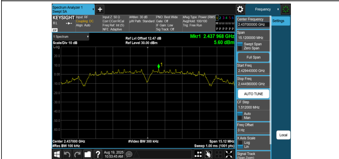
11B-Ant1-2437-PASS
