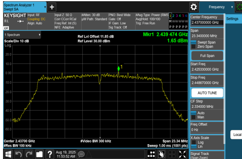
11G-Ant2-2437-PASS
