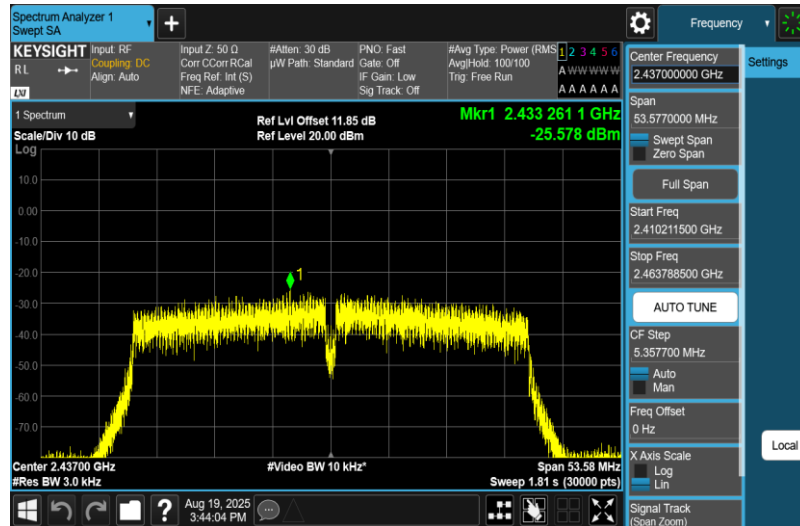
11N40MIMO-Ant2-2437-PASS
