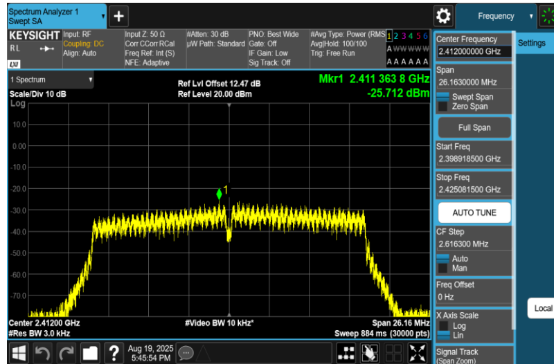
11N20MIMO-Ant1-2412-PASS
