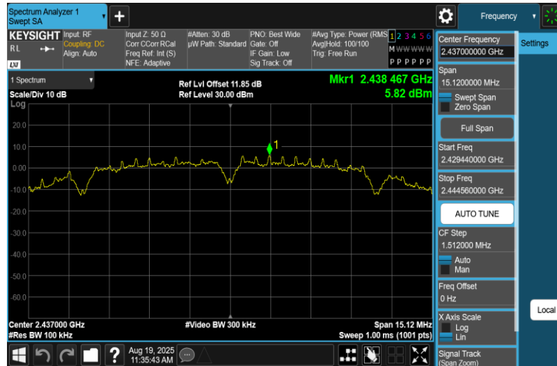
11B-Ant2-2437-PASS
