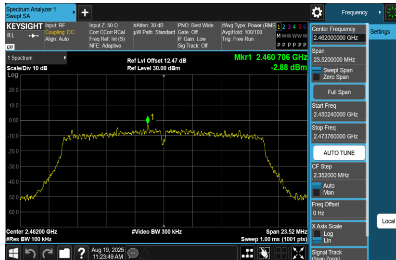
11G-Ant1-2462-PASS
