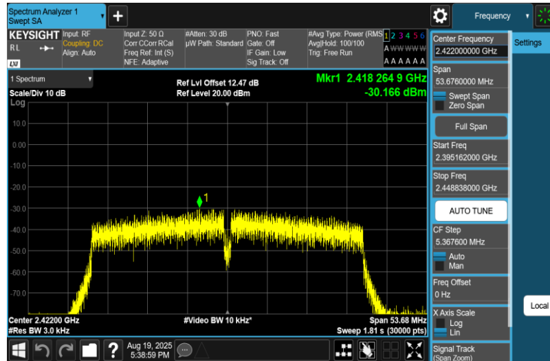
11N40MIMO-Ant1-2422-PASS
