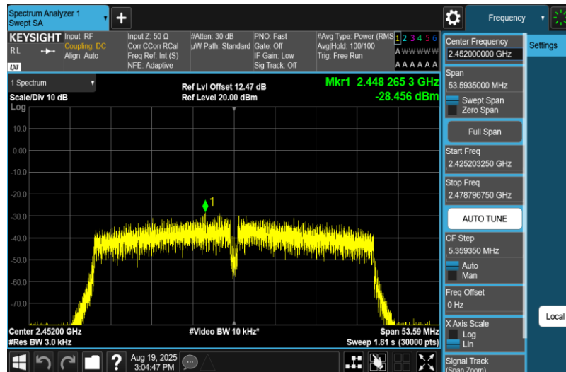
11N40MIMO-Ant1-2452-PASS
