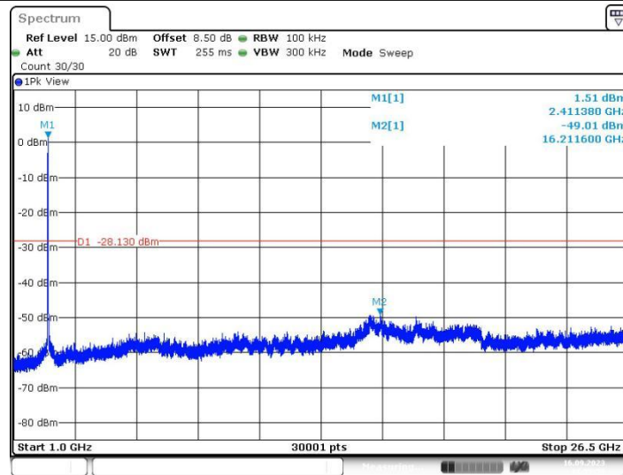
11N20SISO_Ant2_2412_1000~26500
