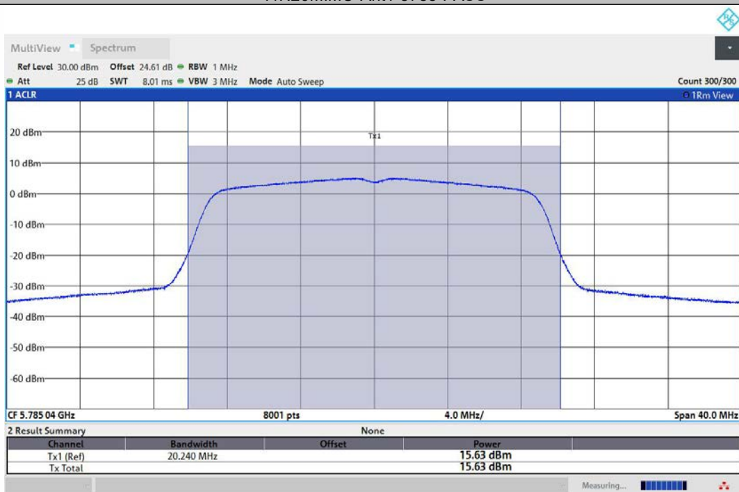
11N20MIMO-Ant2-5785-PASS
