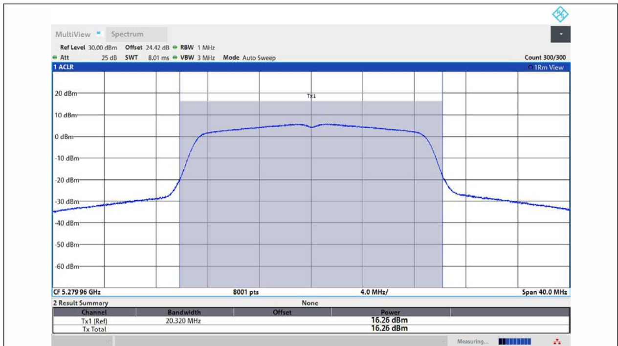
11N20MIMO-Ant2-5280-PASS
