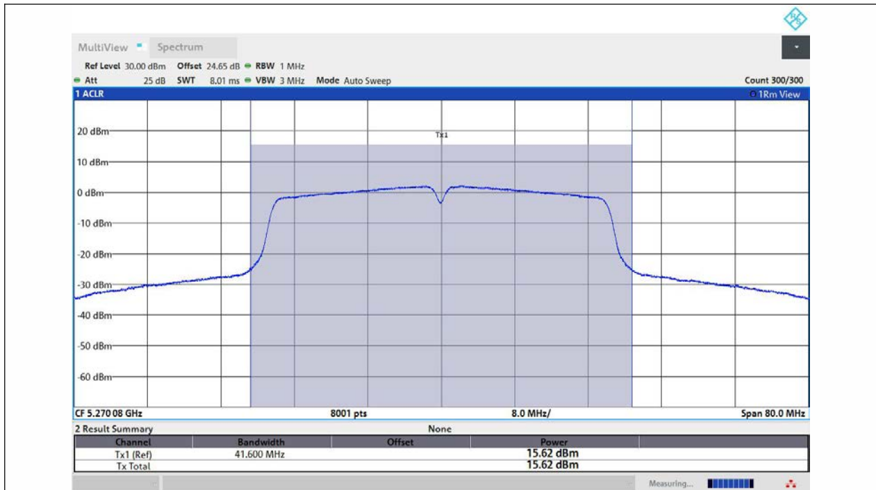
11N40MIMO-Ant1-5270-PASS
