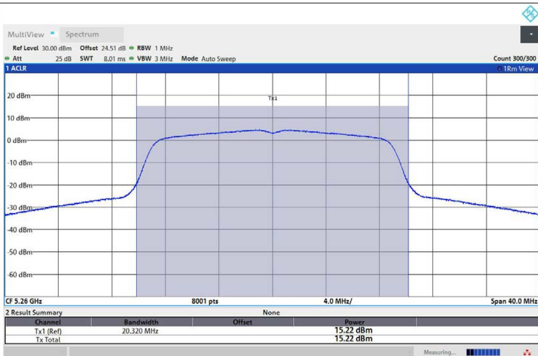
11AC20MIMO-Ant1-5260-PASS
