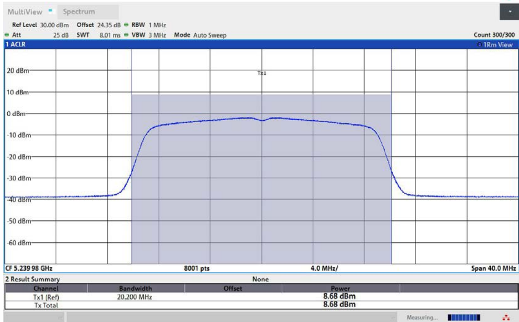
11AC20MIMO-Ant2-5240-PASS
