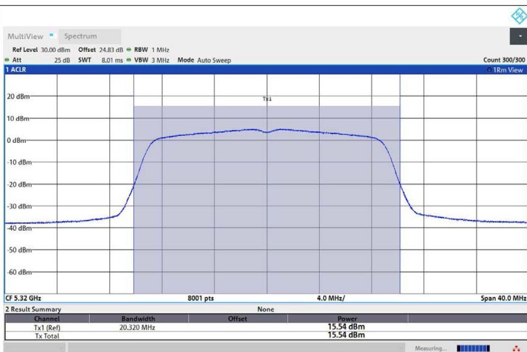
11AC20MIMO-Ant1-5320-PASS
