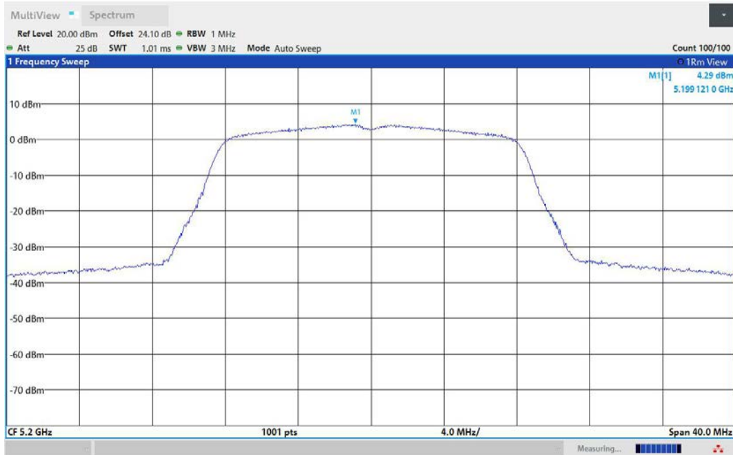
11A-Ant2-5200-PASS
