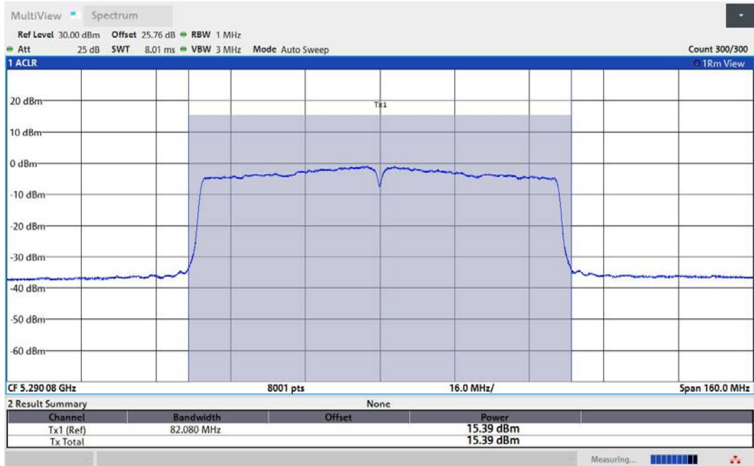
11AC80MIMO-Ant1-5290-PASS
