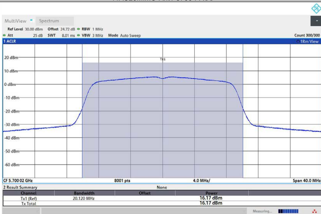
11AC20MIMO-Ant2-5700-PASS
