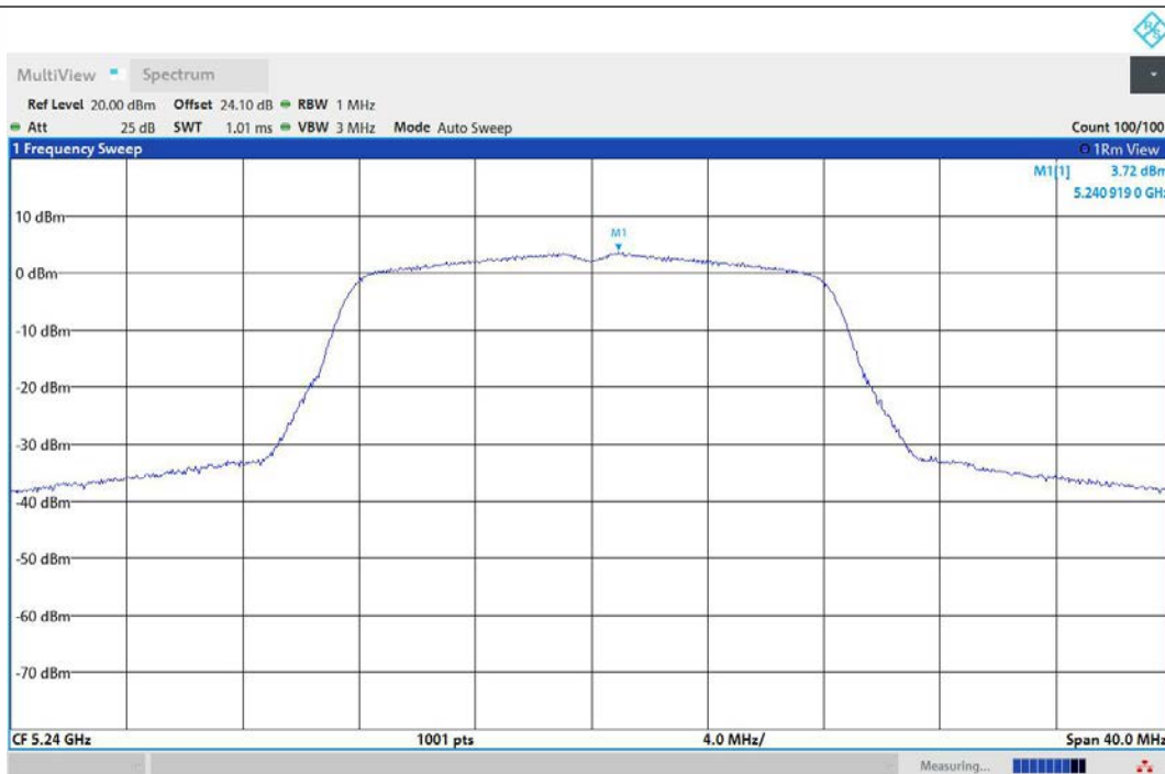
11A-Ant1-5240-PASS
