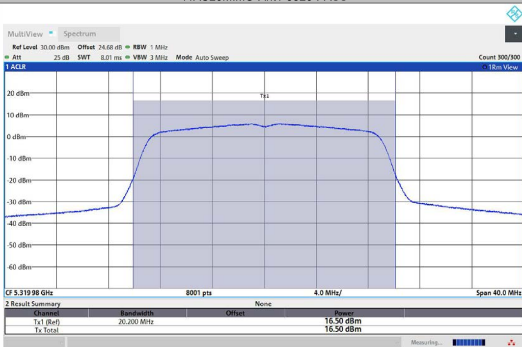
11AC20MIMO-Ant2-5320-PASS
