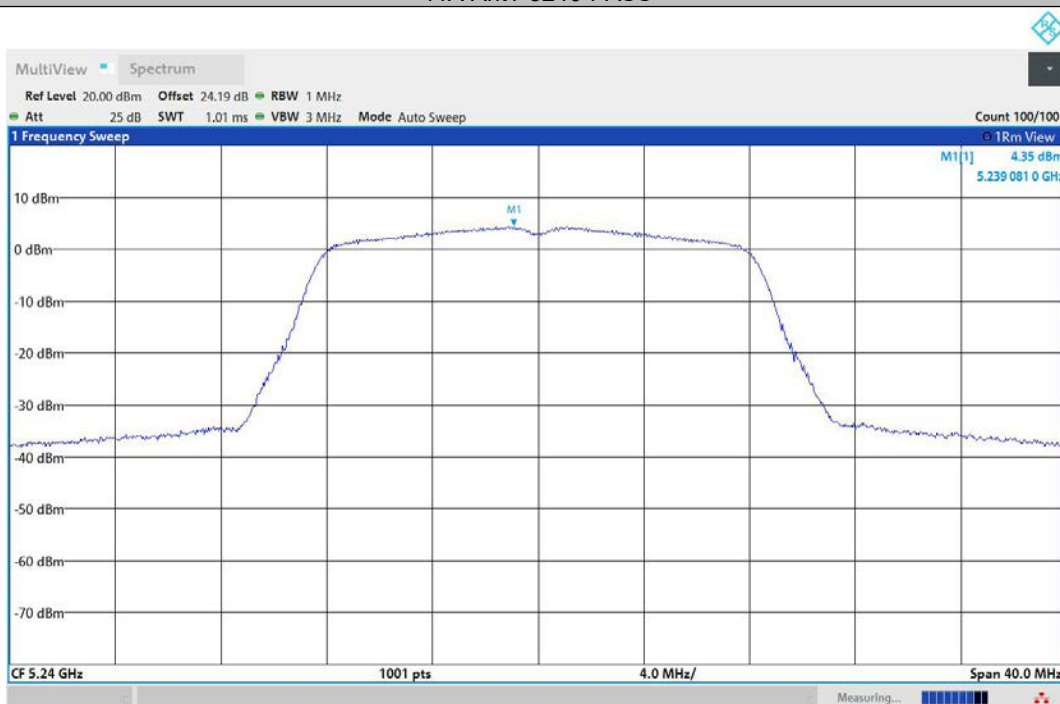
11A-Ant2-5240-PASS
