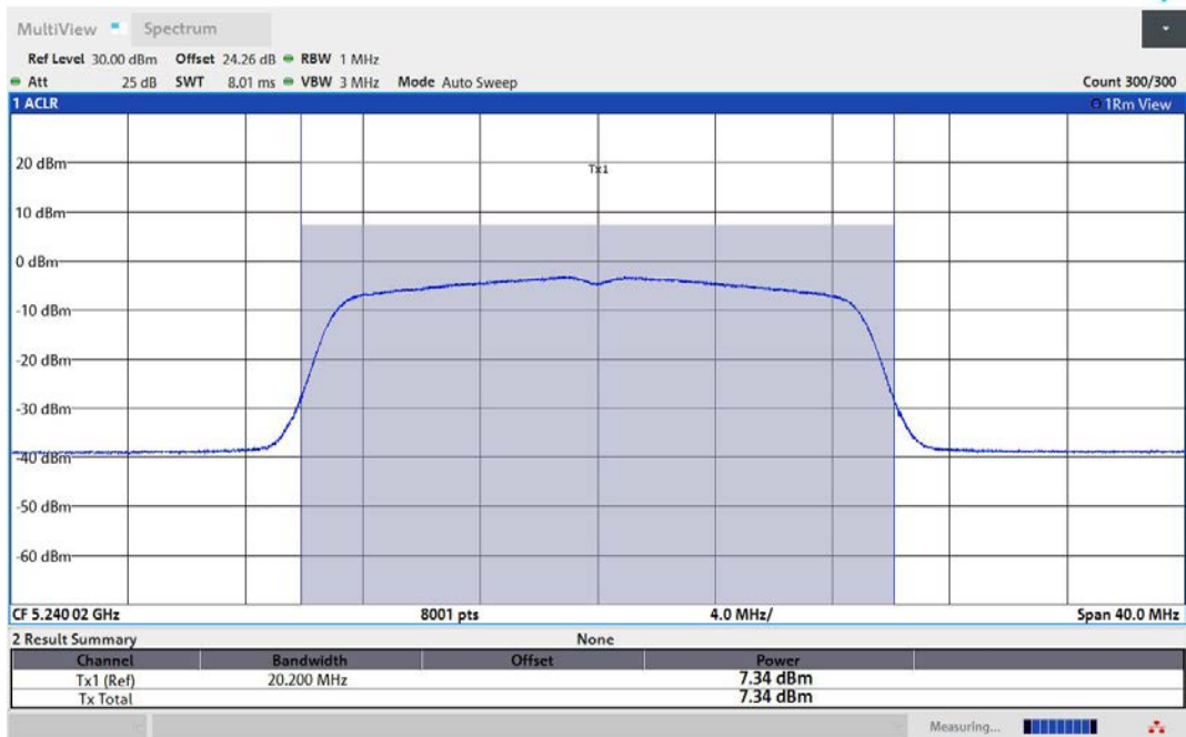
11AC20MIMO-Ant1-5240-PASS
