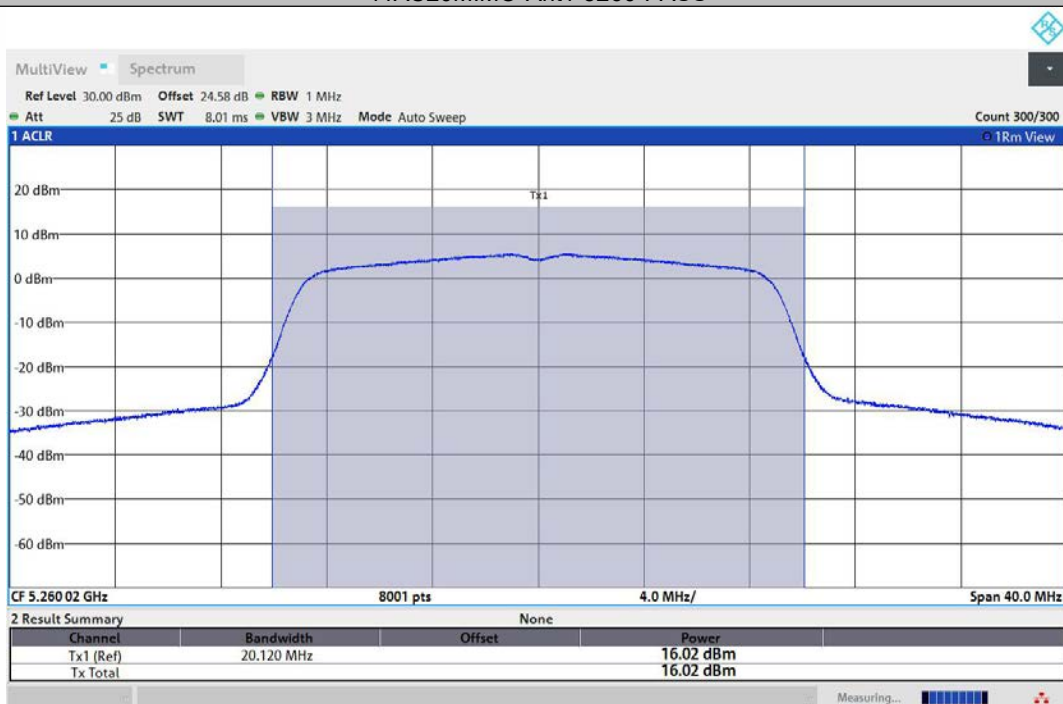
11AC20MIMO-Ant2-5260-PASS
