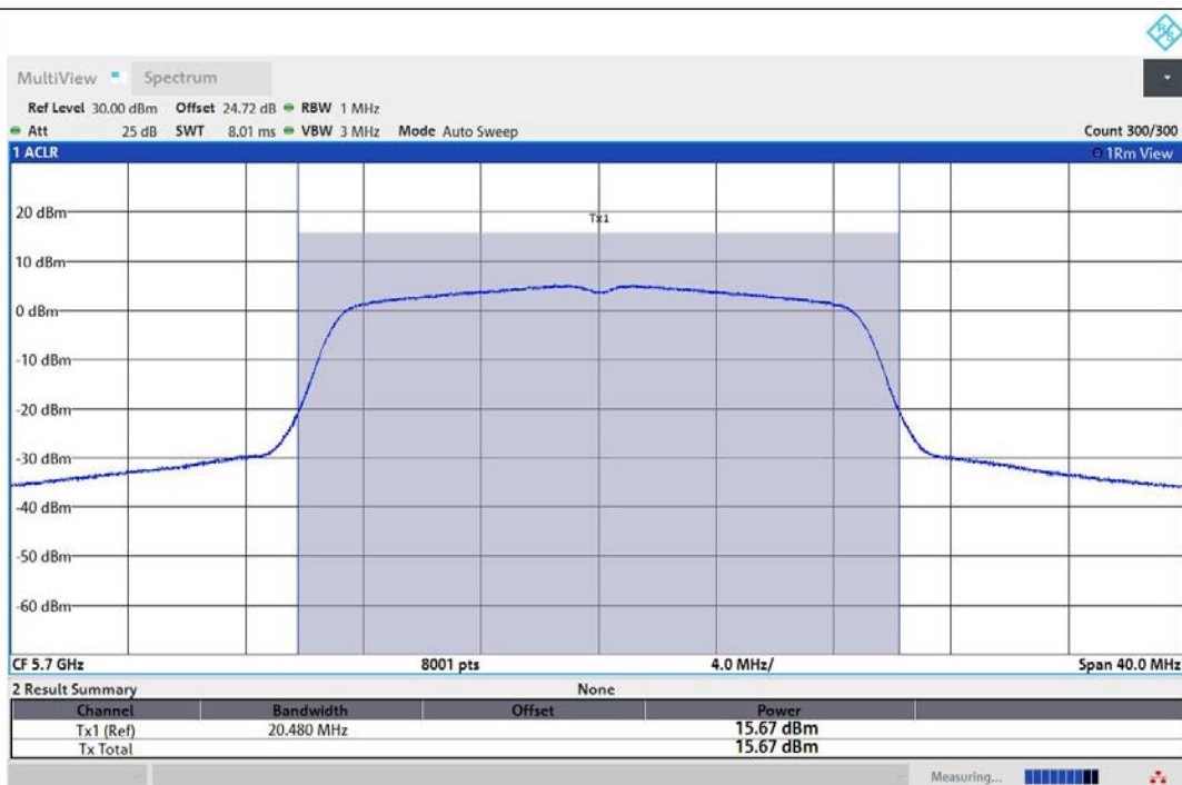
11AC20MIMO-Ant1-5700-PASS
