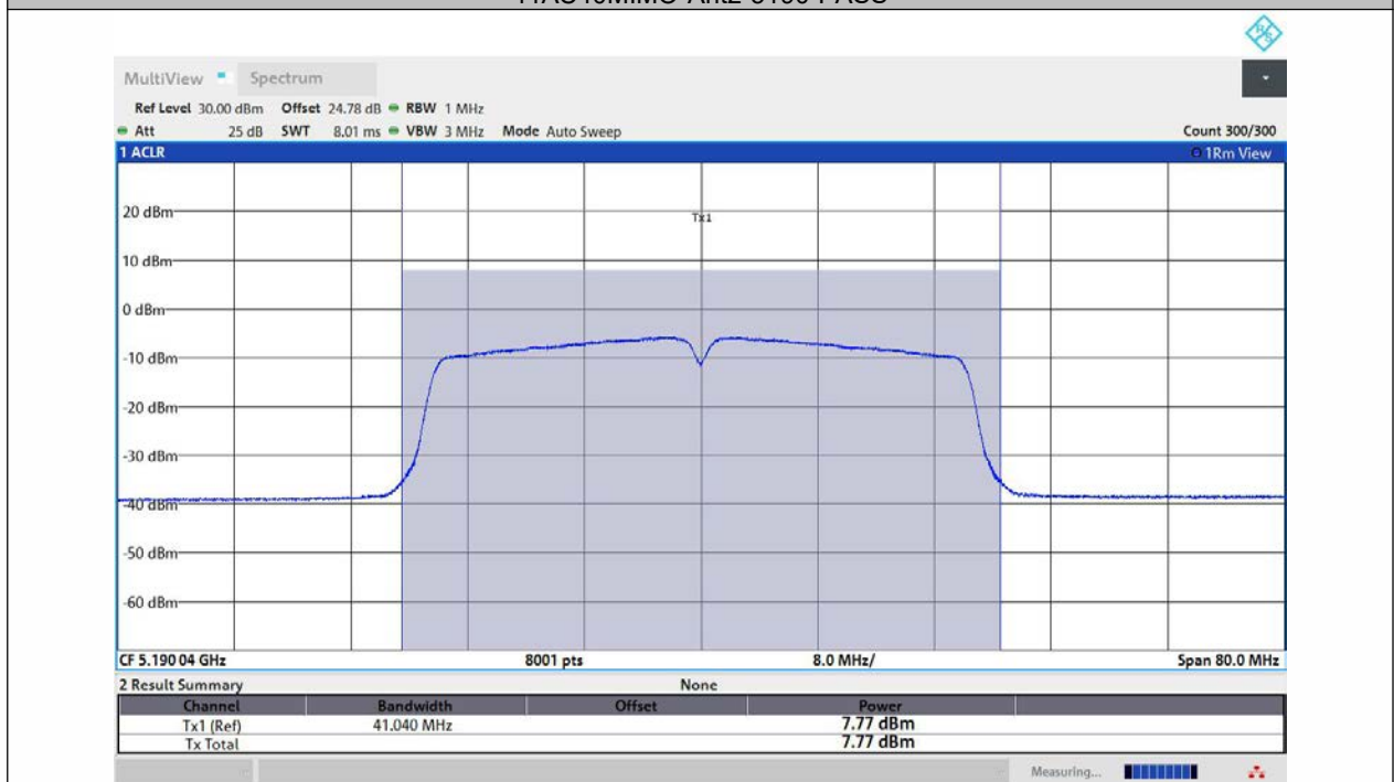
11AC40MIMO-Ant1-5190-PASS
