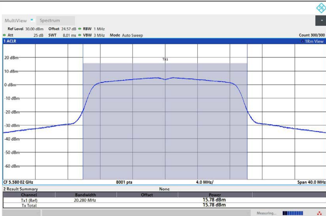
11AC20MIMO-Ant1-5580-PASS
