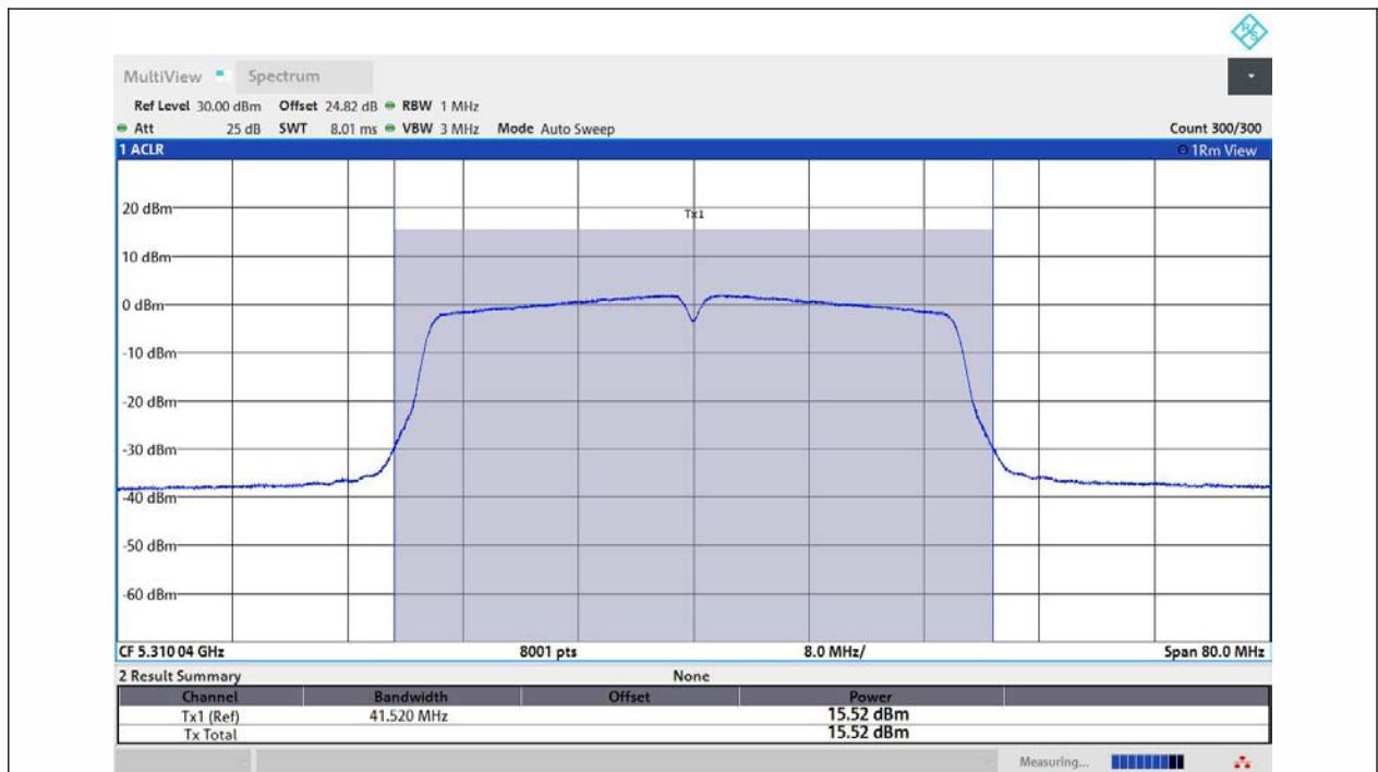
11N40MIMO-Ant1-5310-PASS
