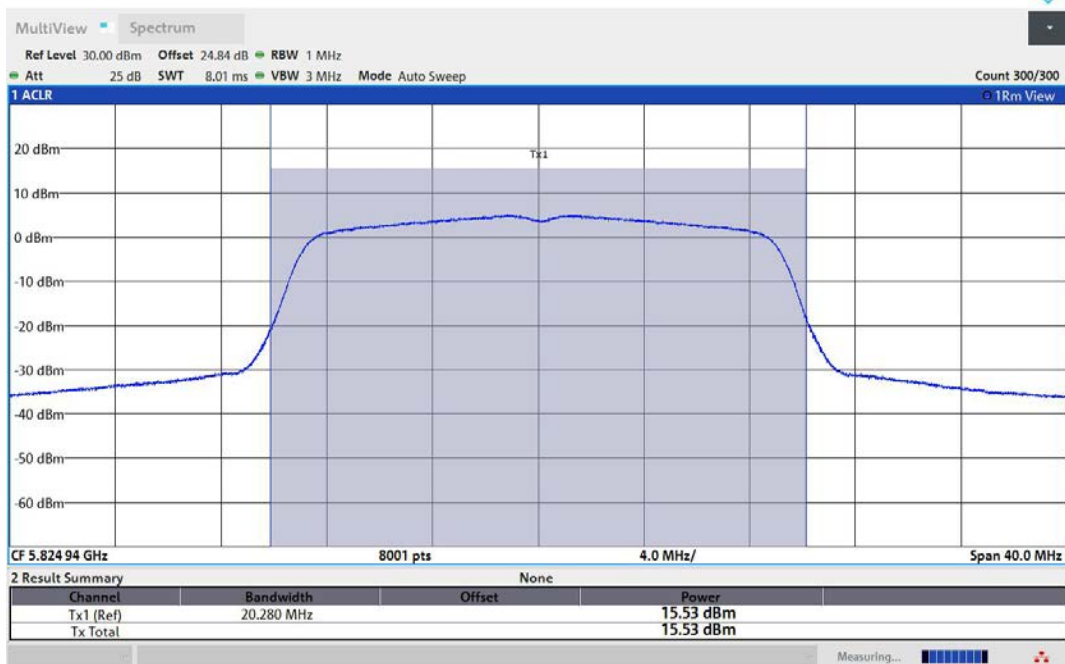
11AC20MIMO-Ant1-5825-PASS
