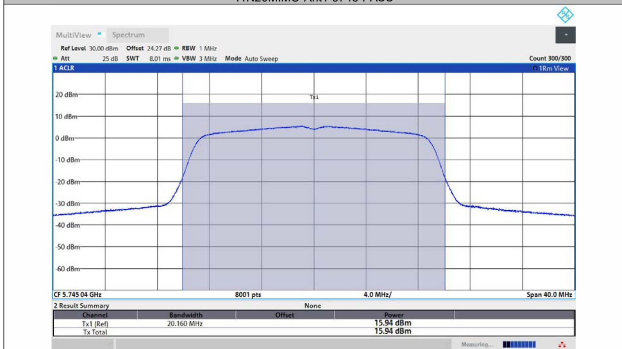
11N20MIMO-Ant2-5745-PASS
