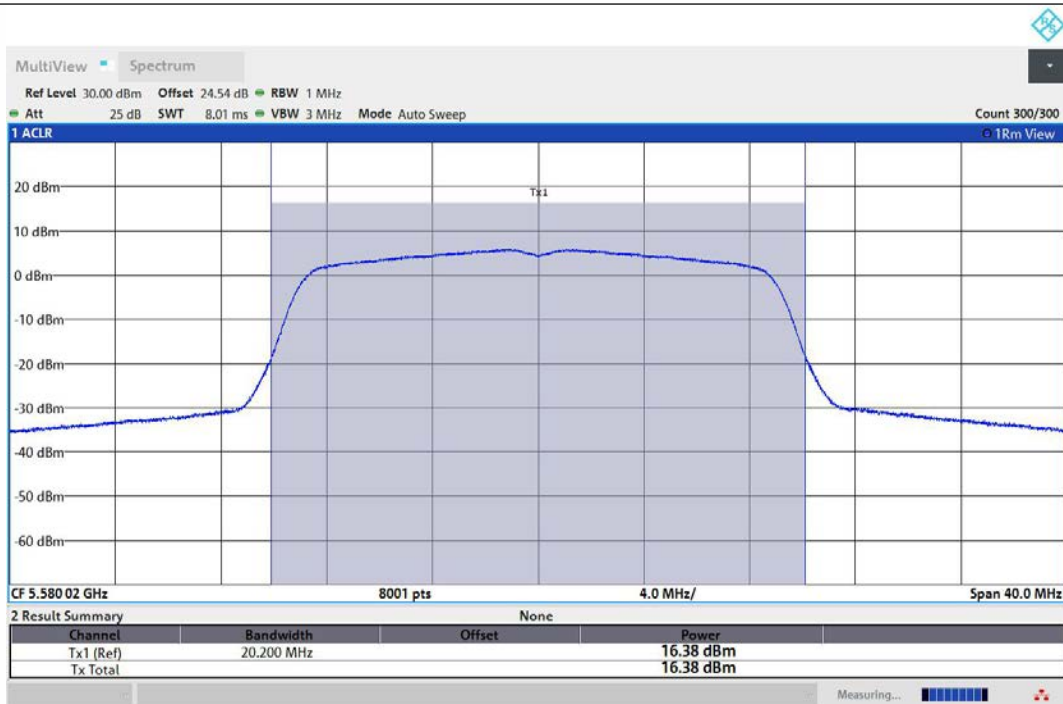
11AC20MIMO-Ant2-5580-PASS
