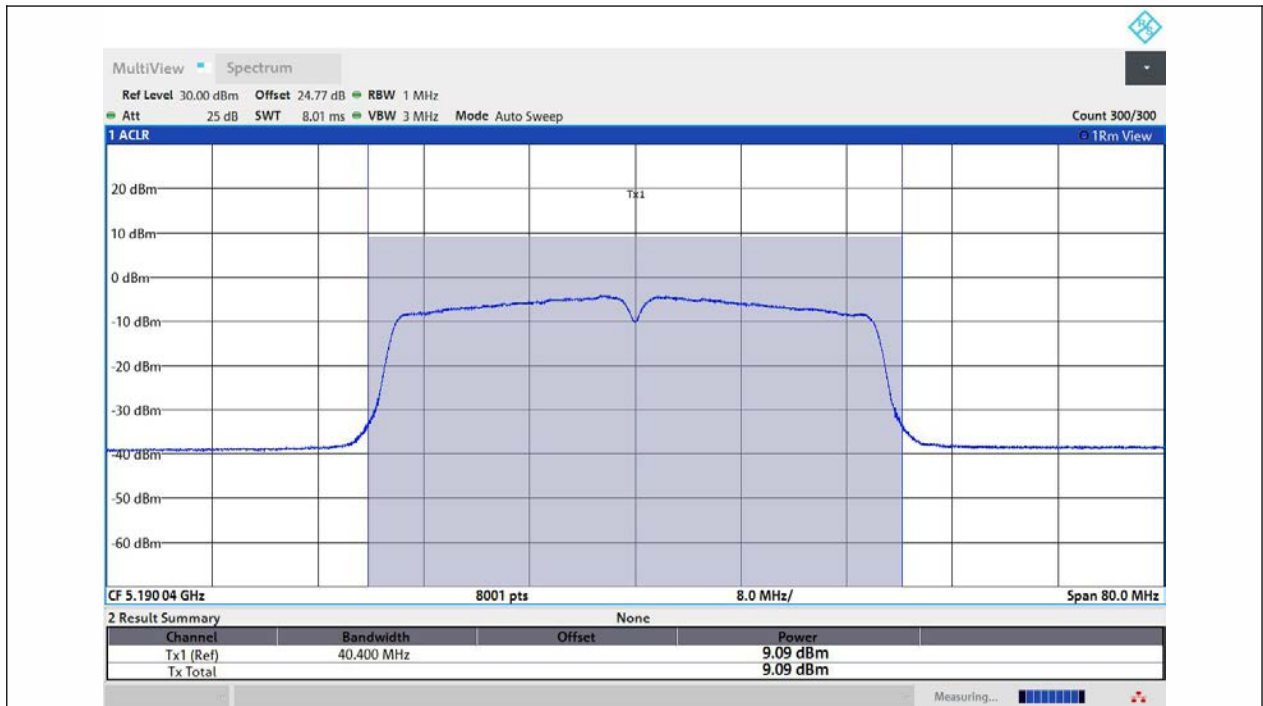
11AC40MIMO-Ant2-5190-PASS
