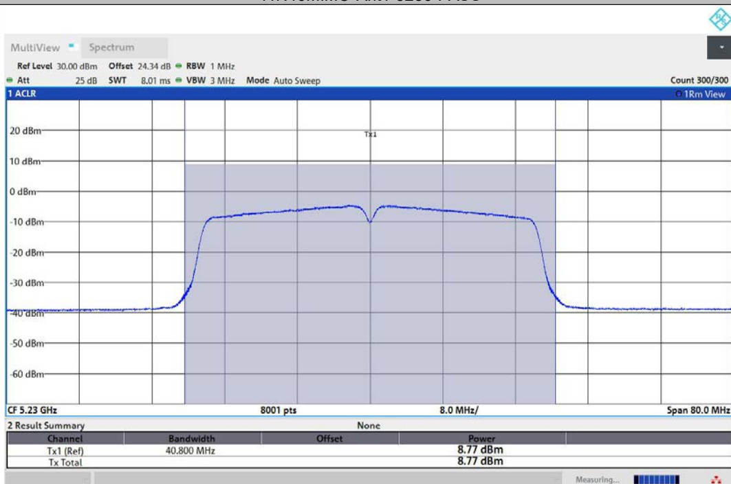
11N40MIMO-Ant2-5230-PASS
