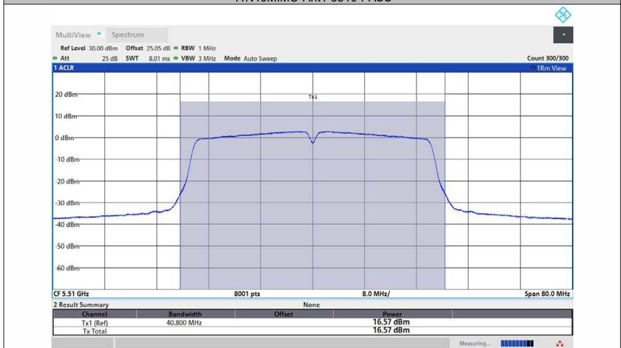
11N40MIMO-Ant2-5510-PASS
