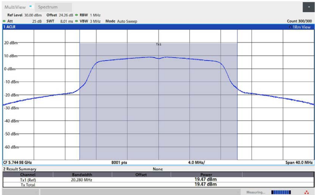
11A-Ant2-5745-PASS
