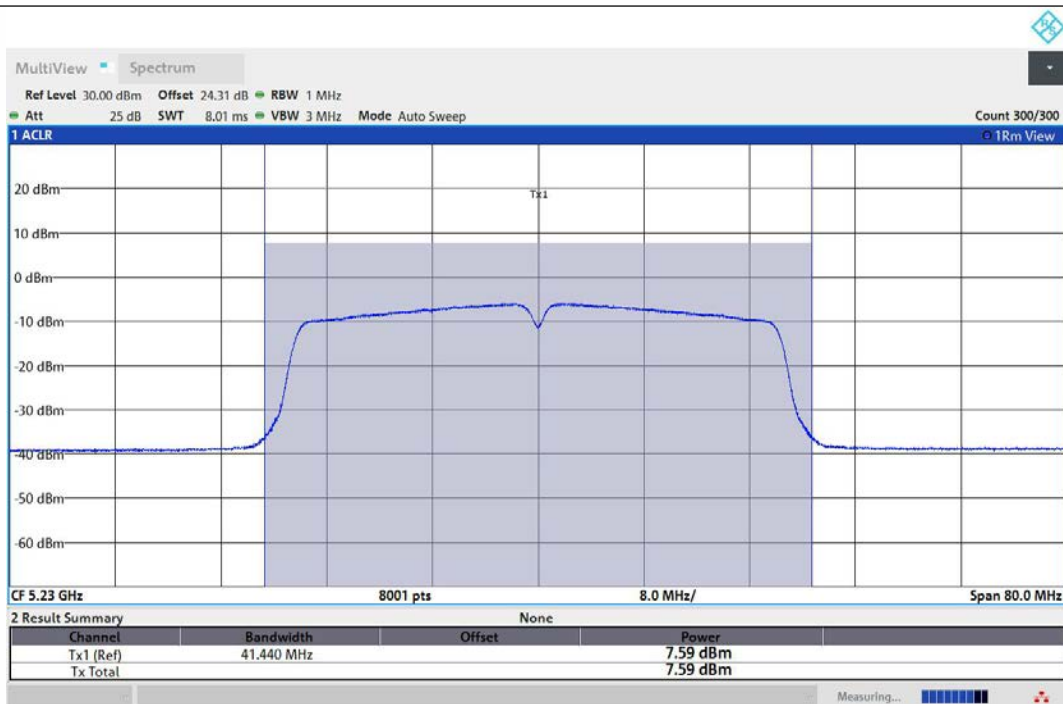
11N40MIMO-Ant1-5230-PASS
