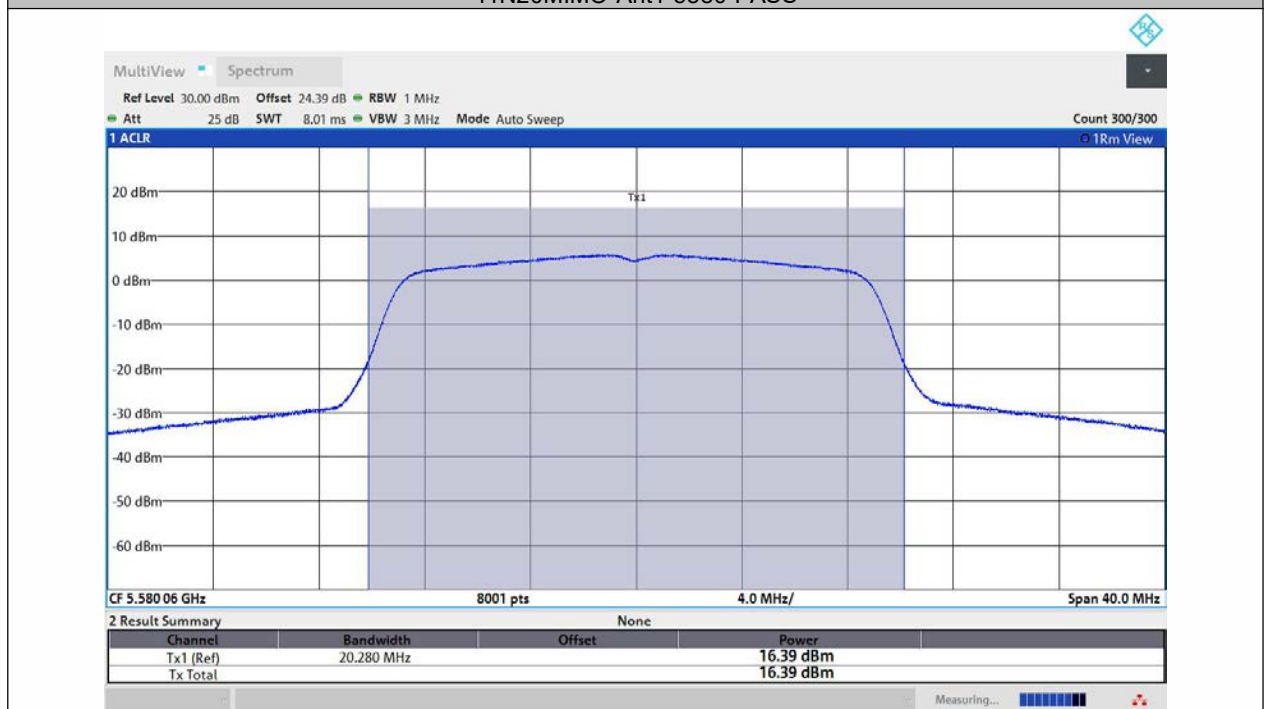
11N20MIMO-Ant2-5580-PASS
