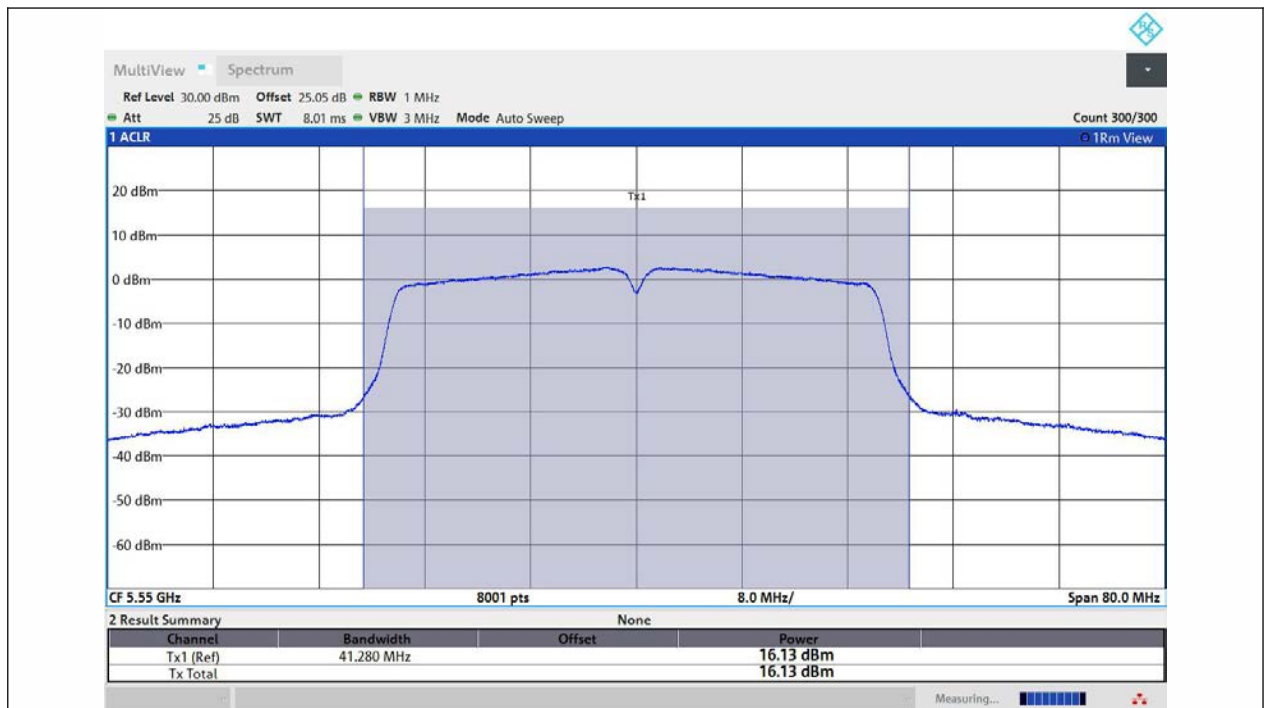
11AC40MIMO-Ant1-5550-PASS
