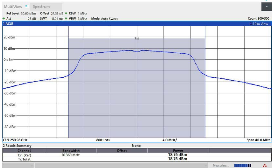
11A-Ant1-5260-PASS
