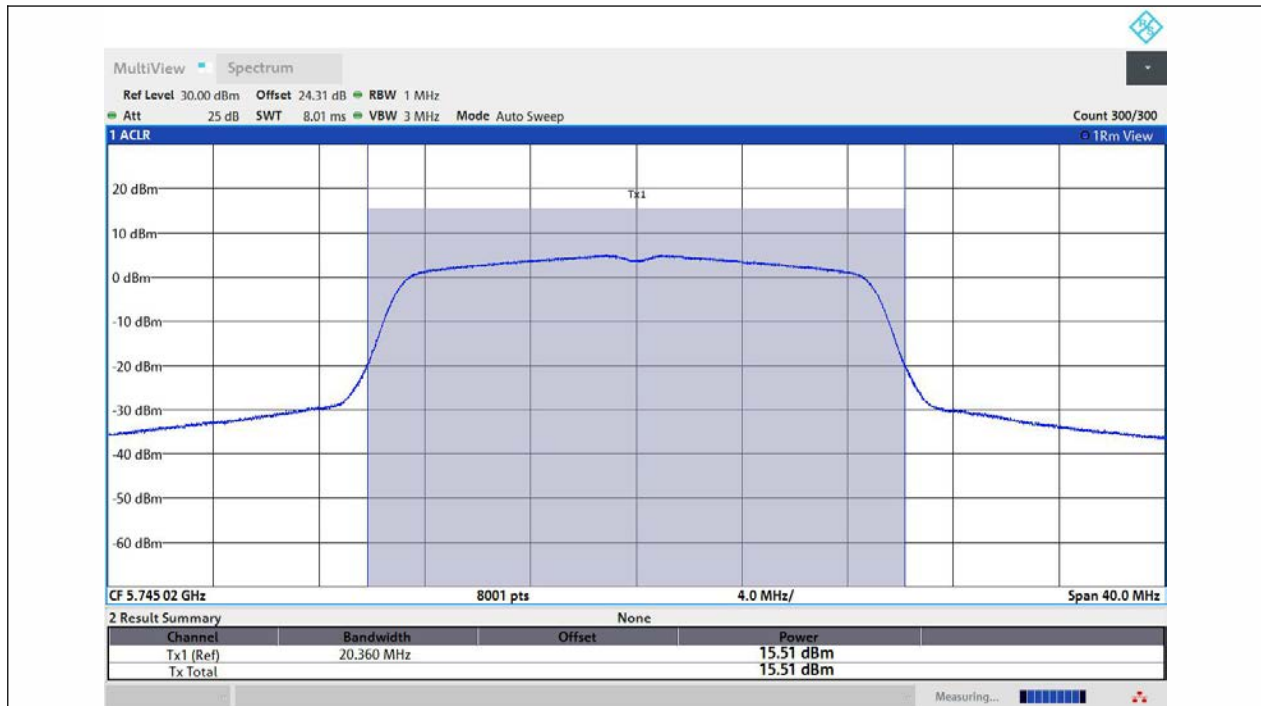
11N20MIMO-Ant1-5745-PASS
