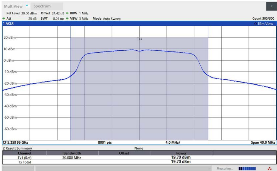
11A-Ant2-5260-PASS
