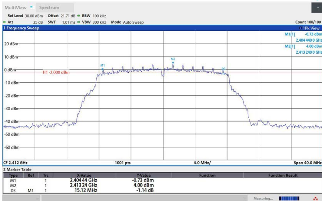
11G-Ant1-2412-PASS
