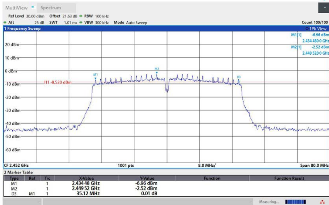
11N40MIMO-Ant1-2452-PASS
