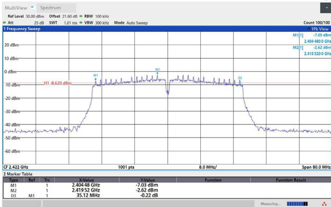
11N40MIMO-Ant1-2422-PASS
