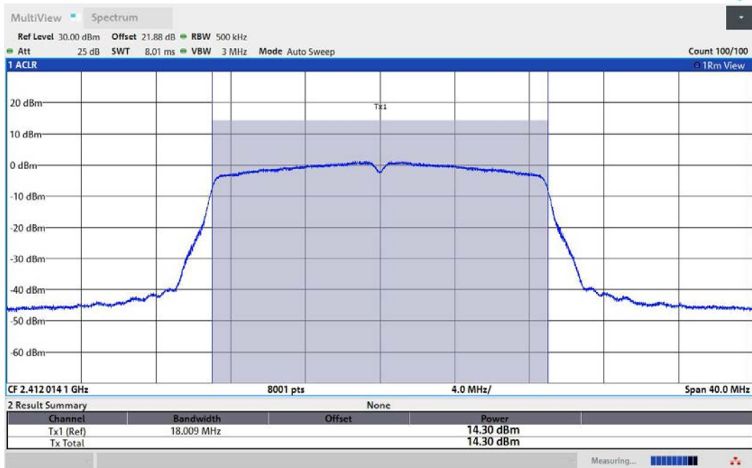
11N20MIMO-Ant1-2412-PASS
