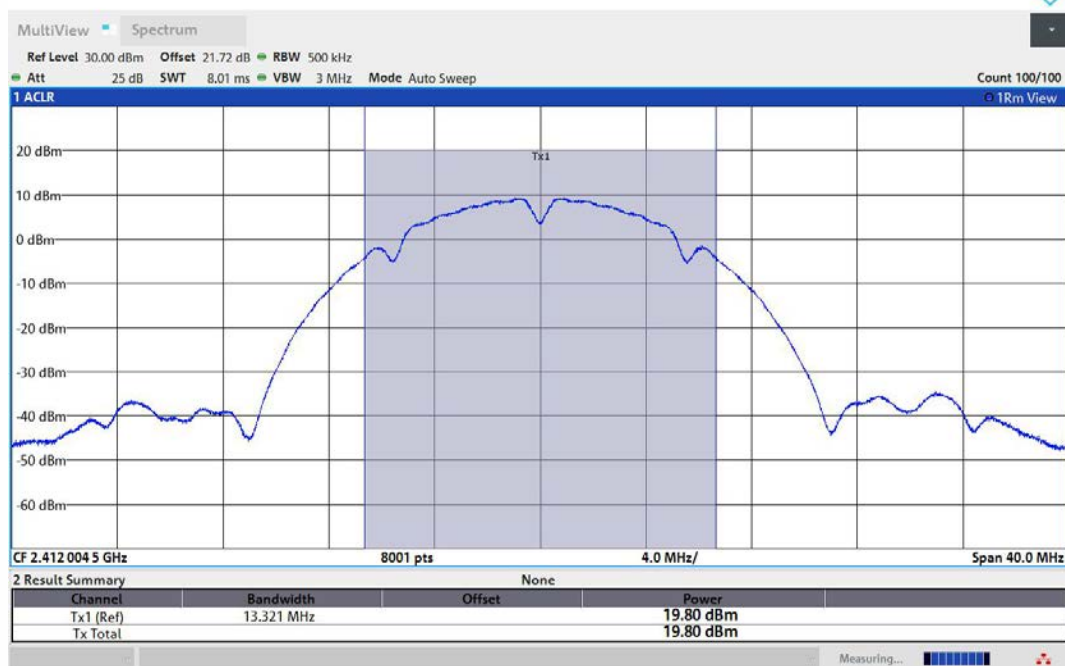
11B-Ant2-2412-PASS
