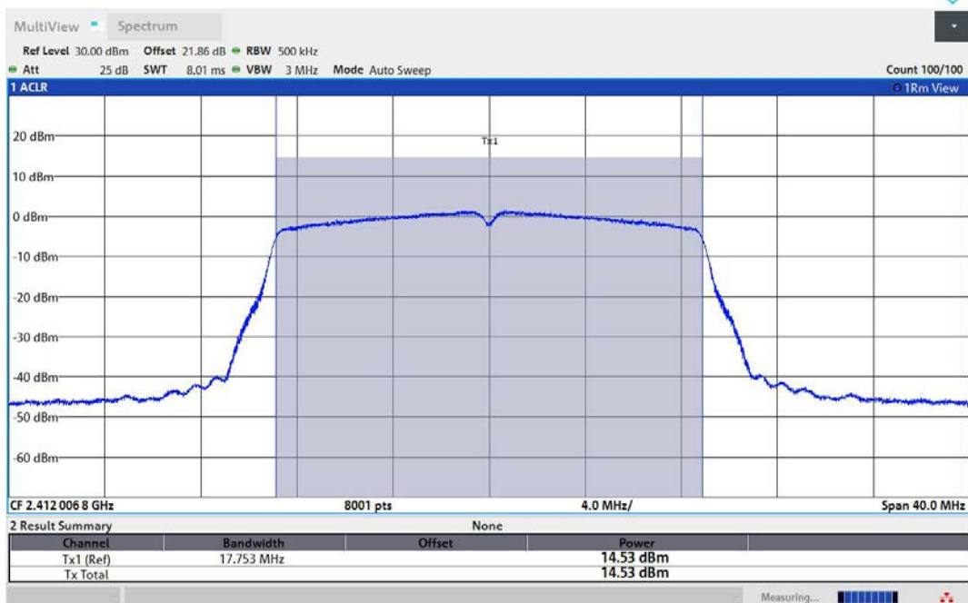
11N20MIMO-Ant2-2412-PASS
