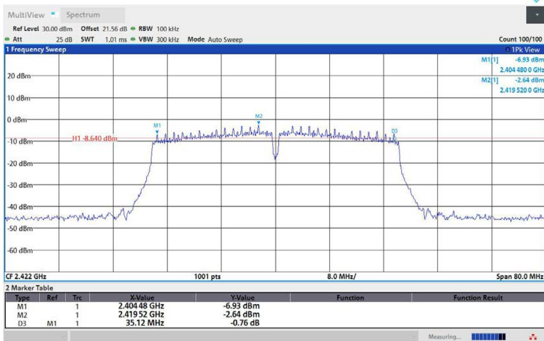
11N40MIMO-Ant2-2422-PASS
