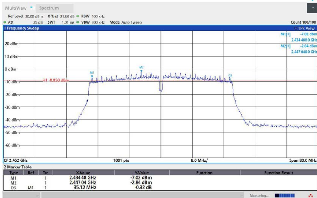
11N40MIMO-Ant2-2452-PASS
