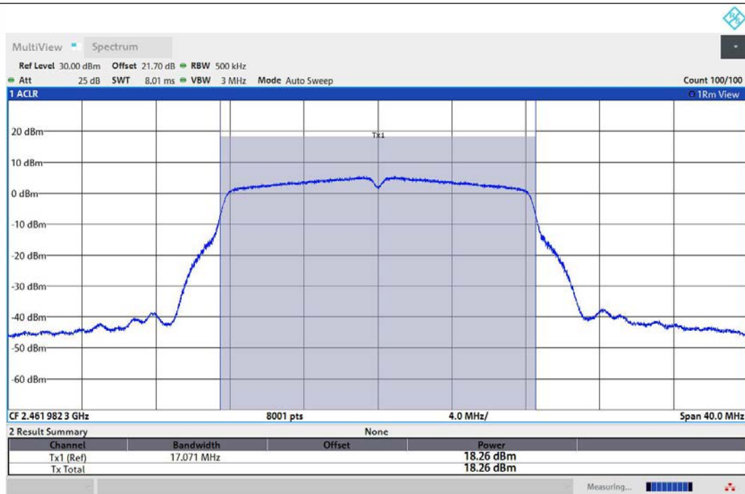
11G-Ant2-2462-PASS
