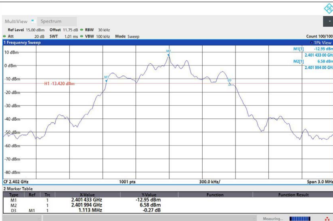
3DH5-Ant1-2402
