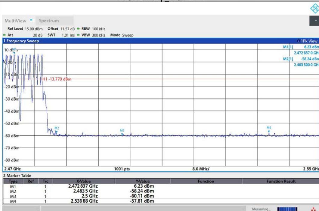
DH5-Ant1-Hop_2480-PASS
