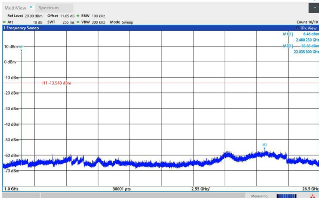
2DH5-Ant1-2480-1000~26500-PASS
