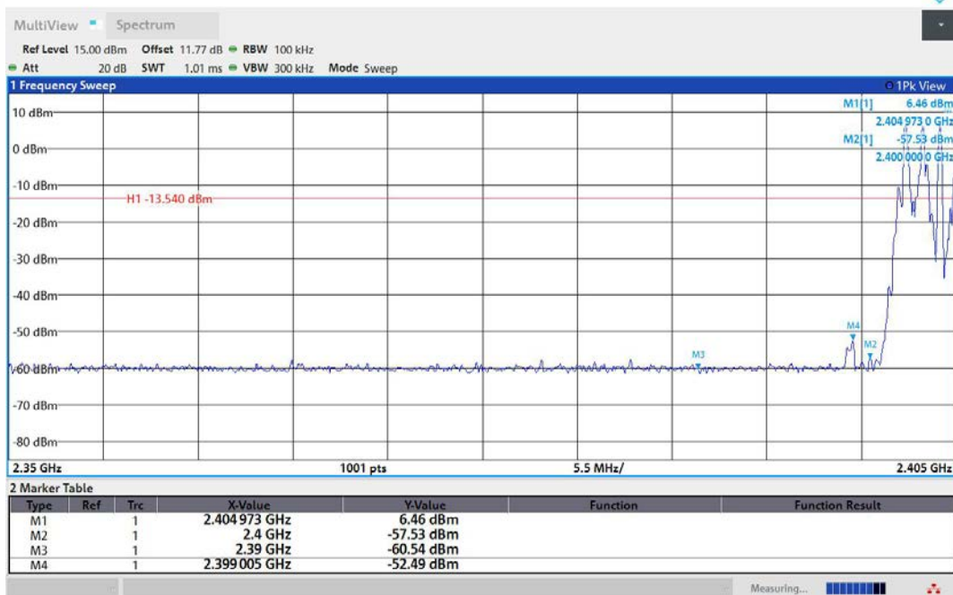
3DH5-Ant1-Hop_2402-PASS
