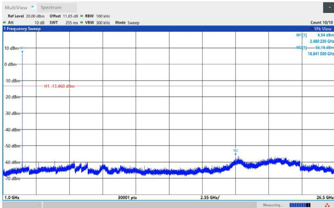
3DH5-Ant1-2480-1000~26500-PASS
