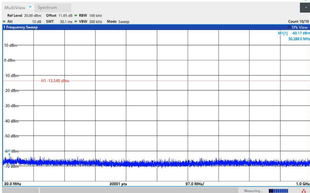
2DH5-Ant1-2480-30~1000-PASS
