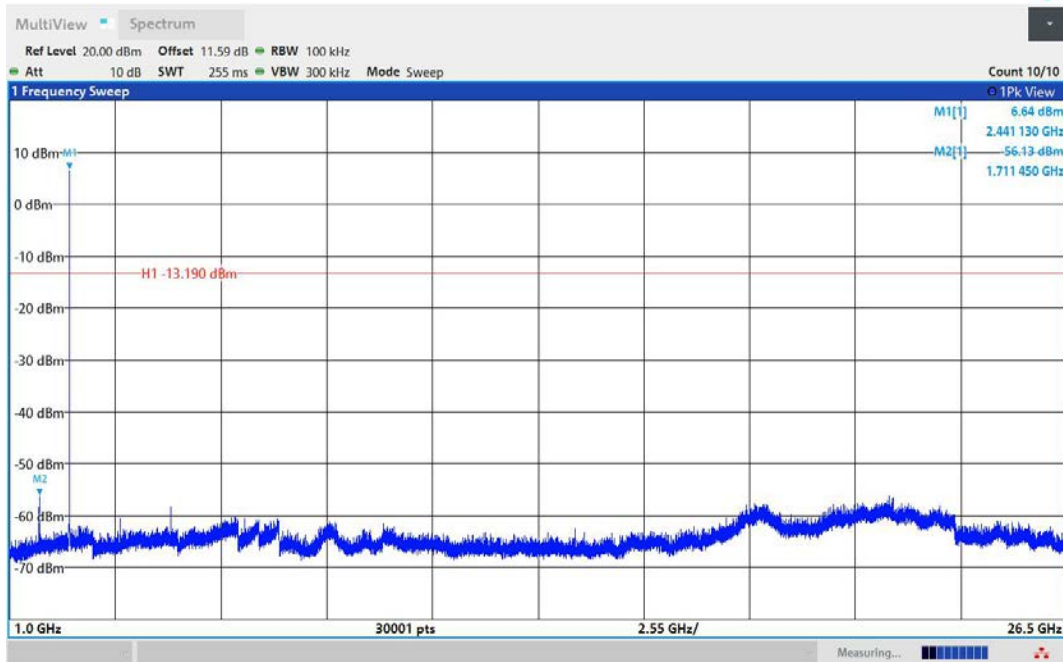
2DH5-Ant1-2441-1000~26500-PASS
