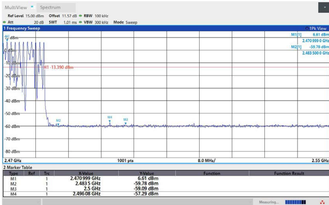
3DH5-Ant1-Hop_2480-PASS
