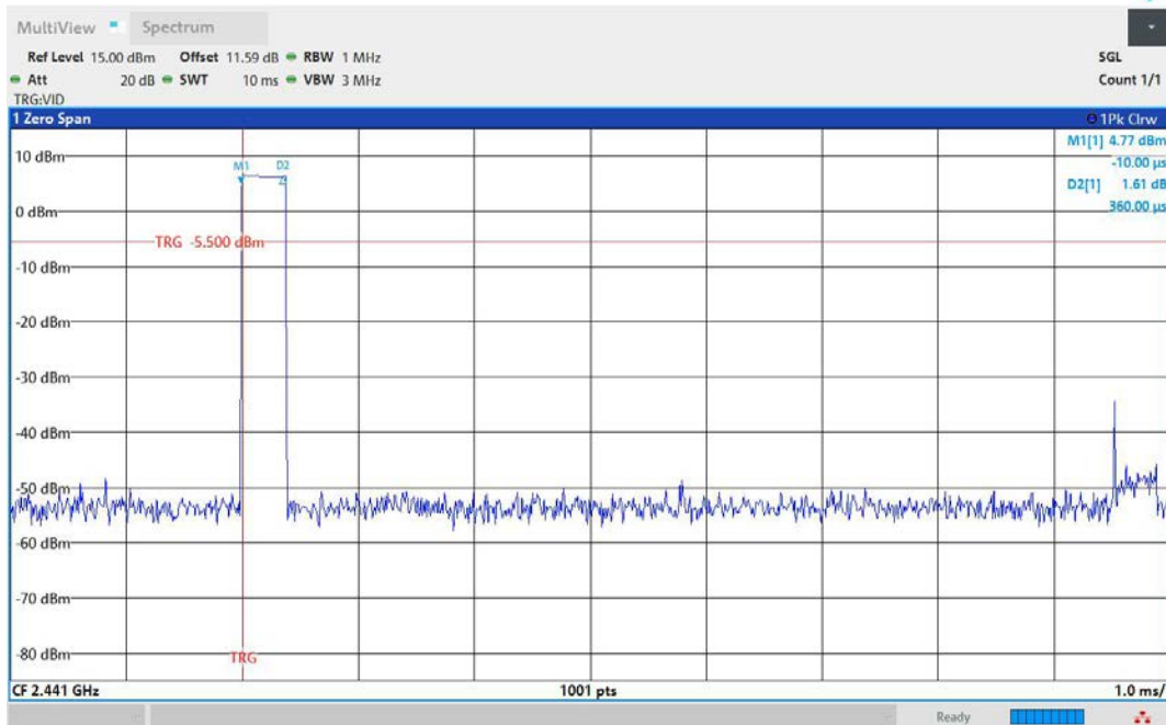
DH1-Ant1-Hop-PASS
