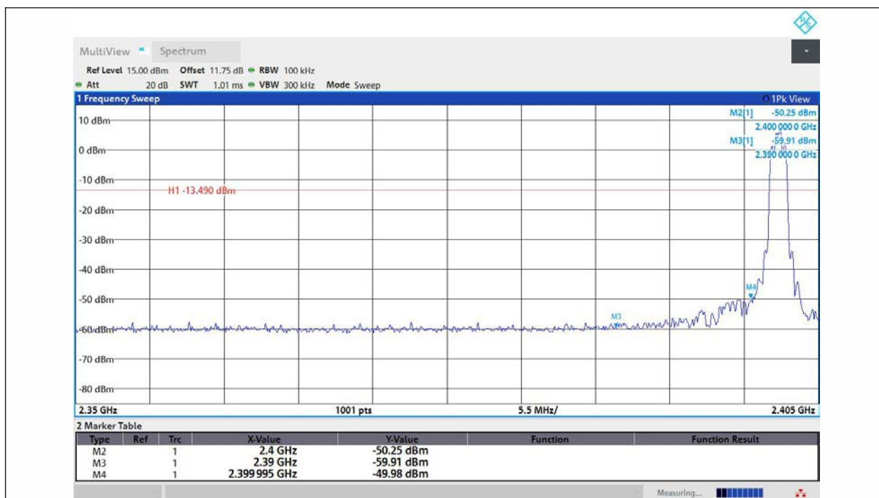
2DH5-Ant1-2402-PASS
