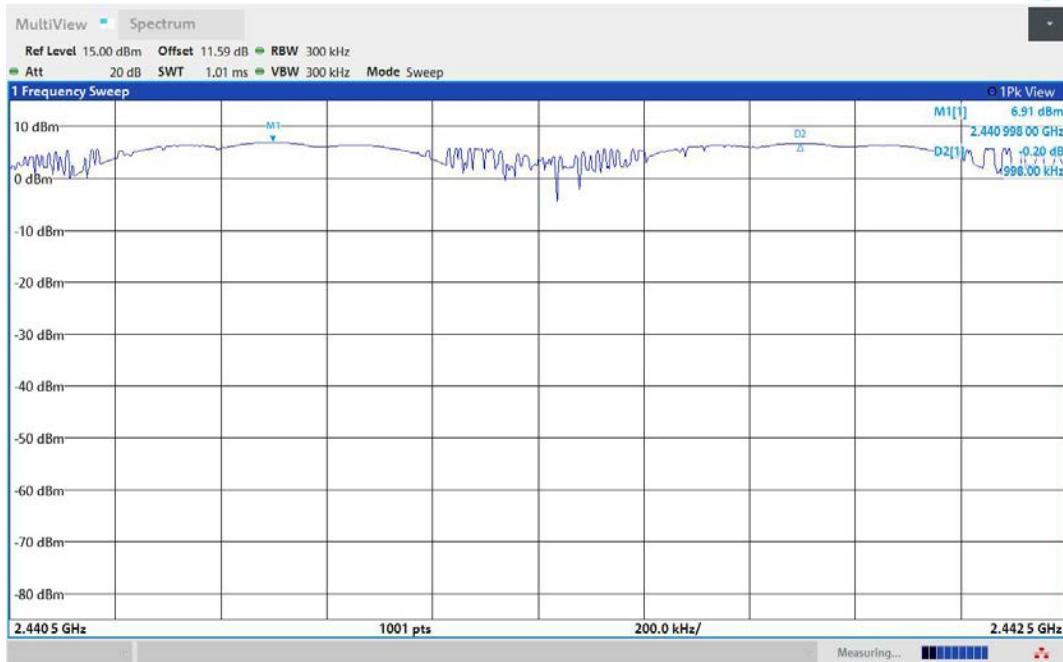
3DH5-Ant1-Hop_2441-PASS
