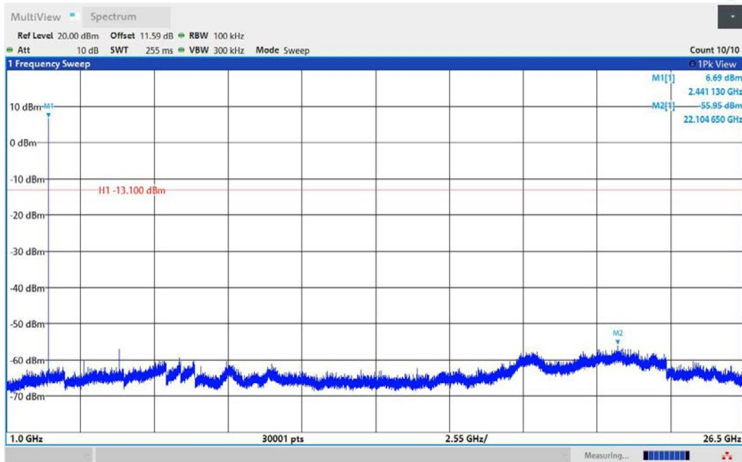
3DH5-Ant1-2441-1000~26500-PASS
