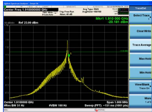
NB-IOT Band 2 BPSK 15kHz 1@0 CH-High
