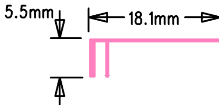
PCB on-board antenna
