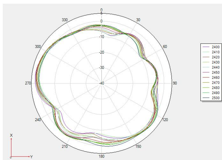
Theta 90 2D
