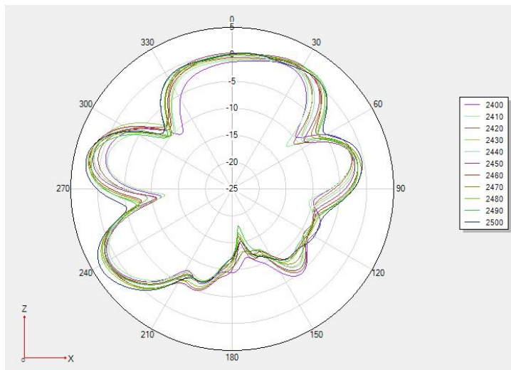
Phi 0 2D
