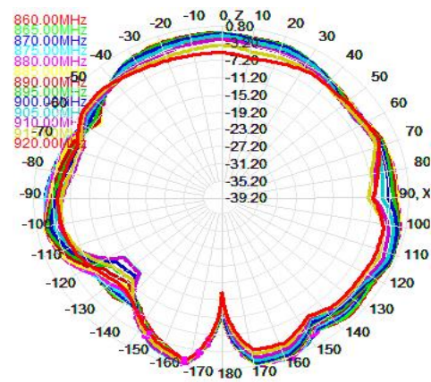
Phi 0 2D
