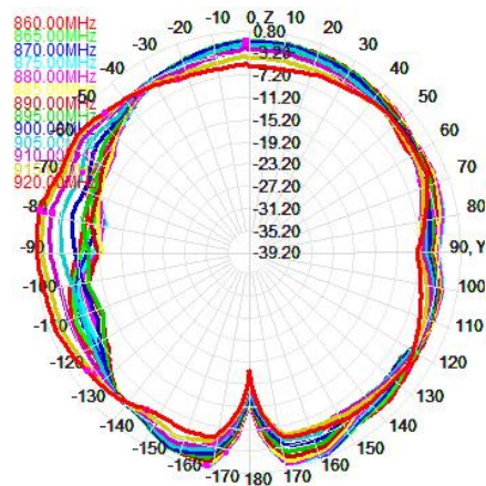
Phi 90 2D
