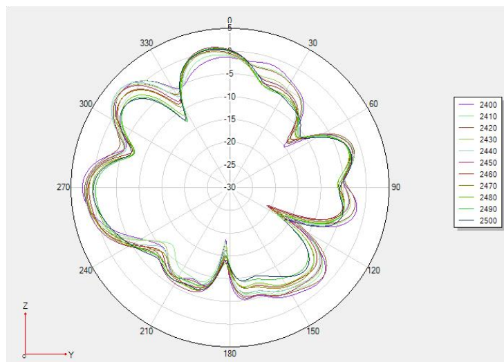
Phi 90 2D
