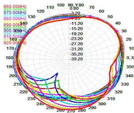
Theta 90 2D
