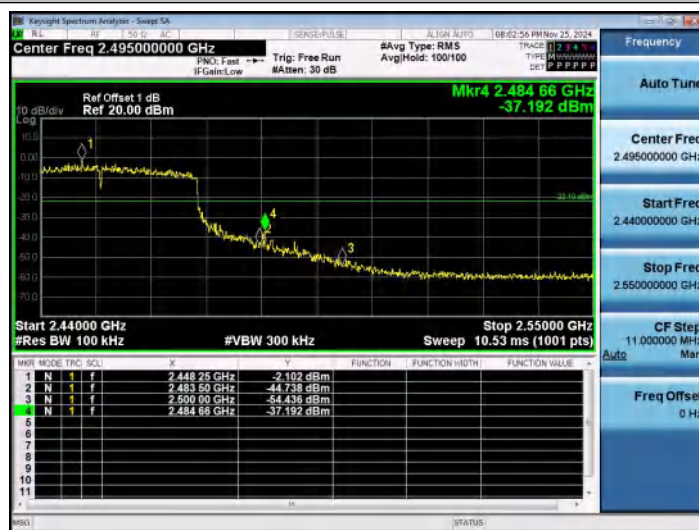
11AX40ISO-Ant1-2452-PASS
