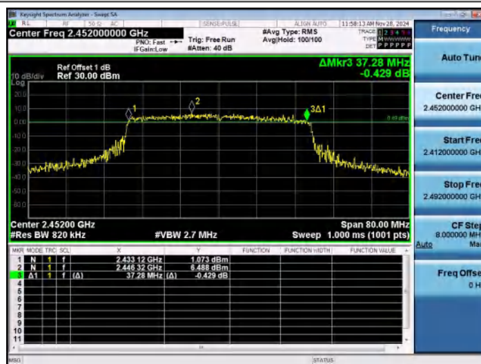
11AX40ISO-Ant1-2452-PASS
