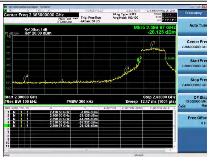
11AX20SISO-Ant1-2412-PASS
