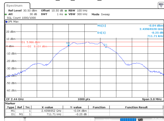
BLE_1M_Middle_Channel
