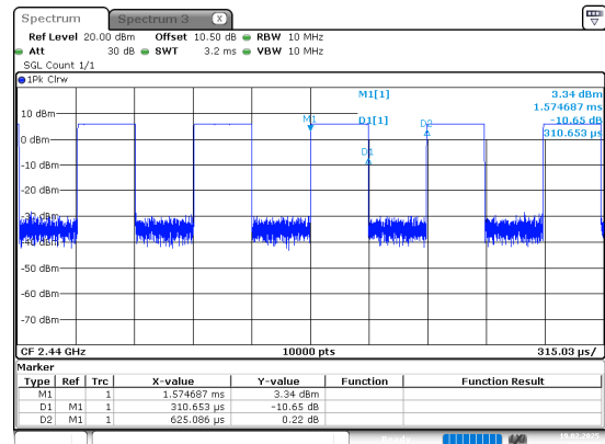
BLE_2M_Middle_Channel
