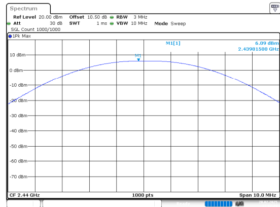
BLE_1M_Middle_Channel
