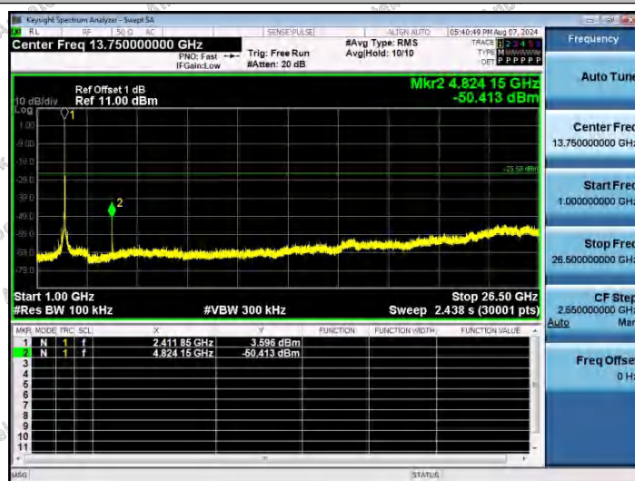
11B-Ant1-2412-1000~26500-PASS
