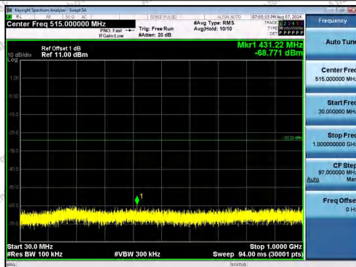
11AX20SISO-Ant1-2437-30~1000-PASS
