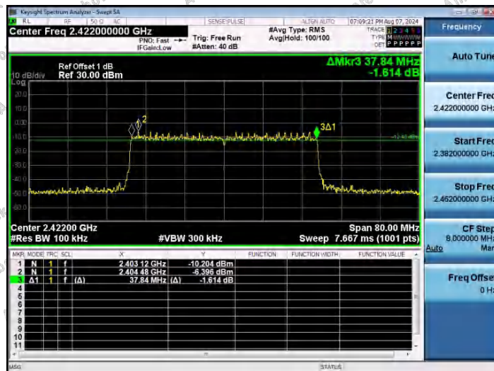
11AX40SISO-Ant1-2422-PASS
