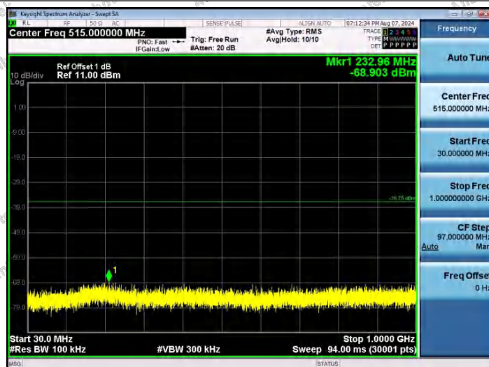
11AX40SISO-Ant1-2437-30~1000-PASS
