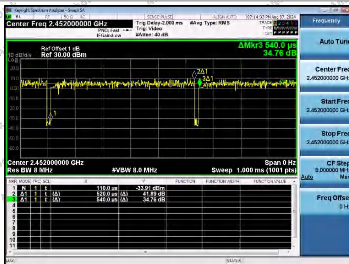
NTNV-11AX40SISO-Ant1-2452
