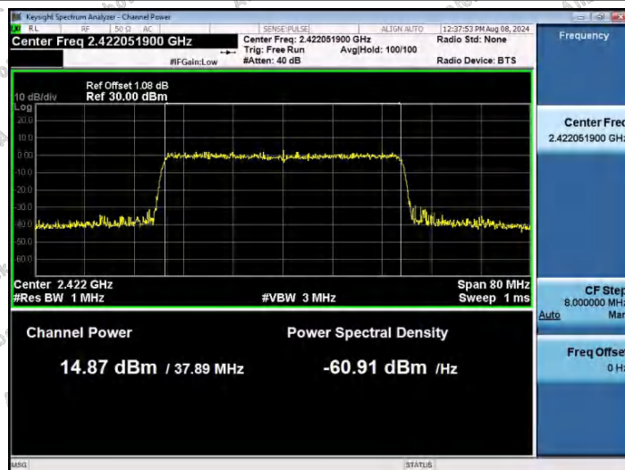
11AX40SISO-Ant1-2422-PASS
