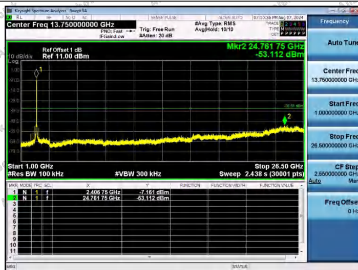
11AX40SISO-Ant1-2422-1000~26500-PASS
