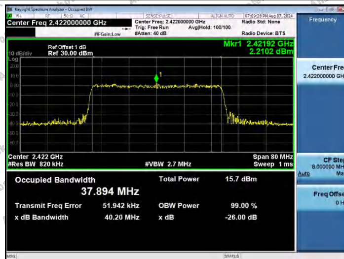
11AX40SISO-Ant1-2422
