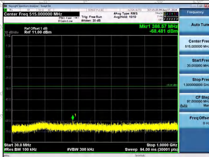
11AX40SISO-Ant1-2452-30~1000-PASS
