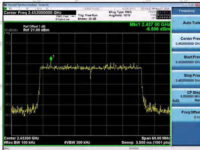
11AX40SISO-Ant1-2452-0~Reference-PASS
