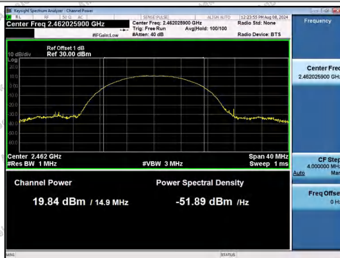
11B-Ant1-2462-PASS
