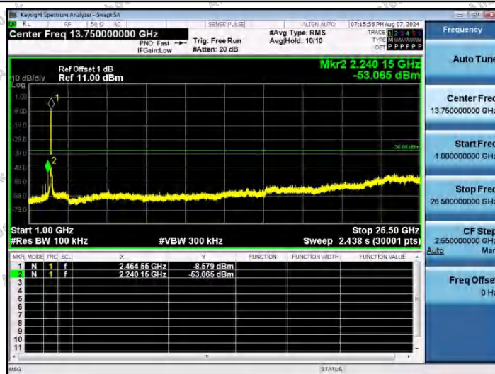
11AX40SISO-Ant1-2452-1000~26500-PASS
