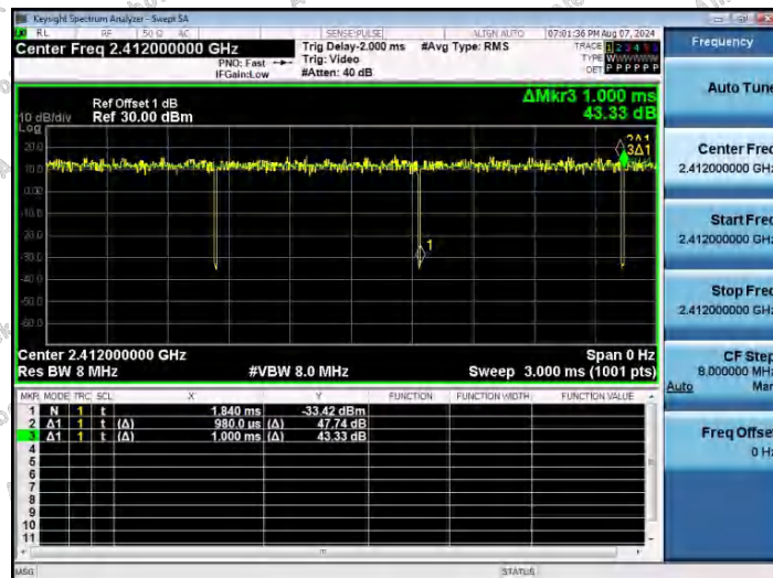
NTNV-11AX20SISO-Ant1-2412
