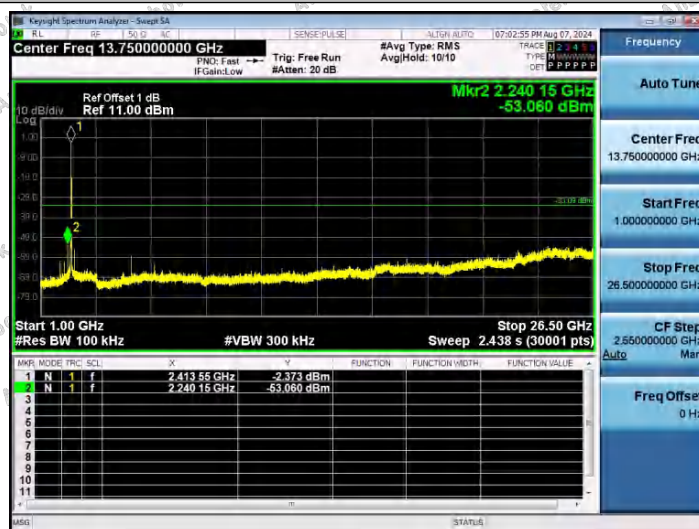
11AX20SISO-Ant1-2412-1000~26500-PASS
