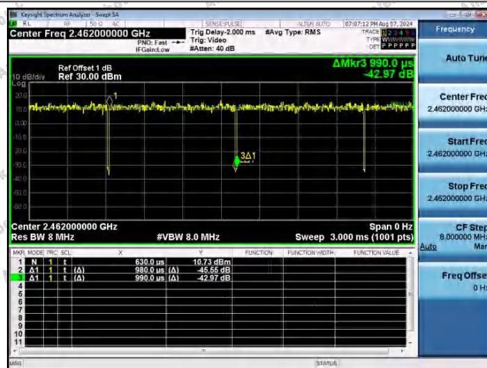
NTNV-11AX20SISO-Ant1-2462
