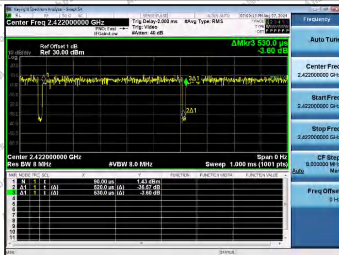
NTNV-11AX40SISO-Ant1-2422
