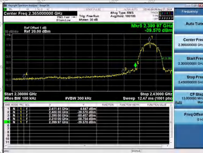
11B-Ant1-2412-PASS
