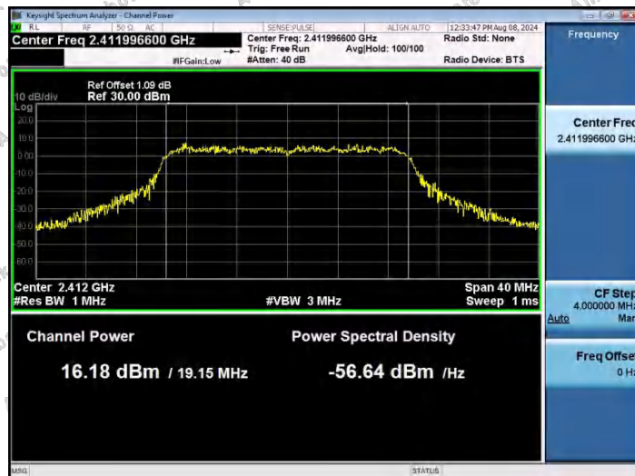
11AX20SISO-Ant1-2412-PASS
