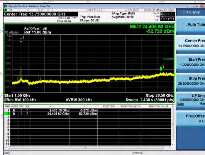
11AX20SISO-Ant1-2437-1000~26500-PASS
