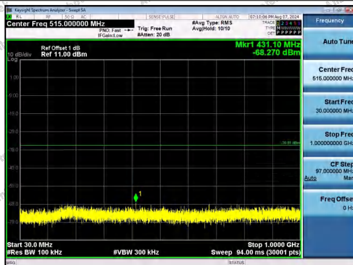
11AX40SISO-Ant1-2422-30~1000-PASS
