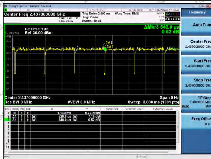
NTNV-11AX40SISO-Ant1-2437
