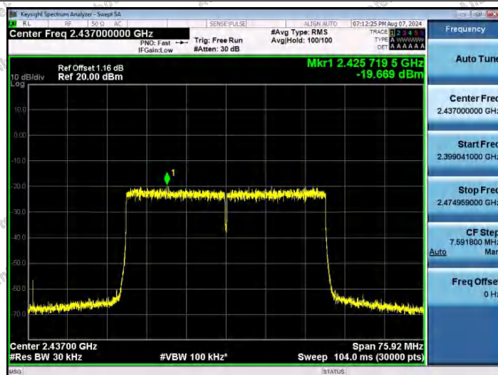
11AX40SISO-Ant1-2437-PASS
