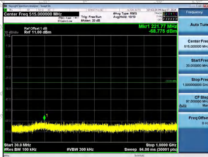
11AX20SISO-Ant1-2412-30~1000-PASS
