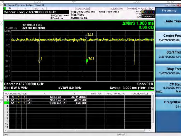
NTNV-11AX20SISO-Ant1-2437
