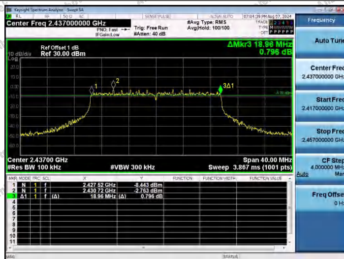
11AX20SISO-Ant1-2437-PASS
