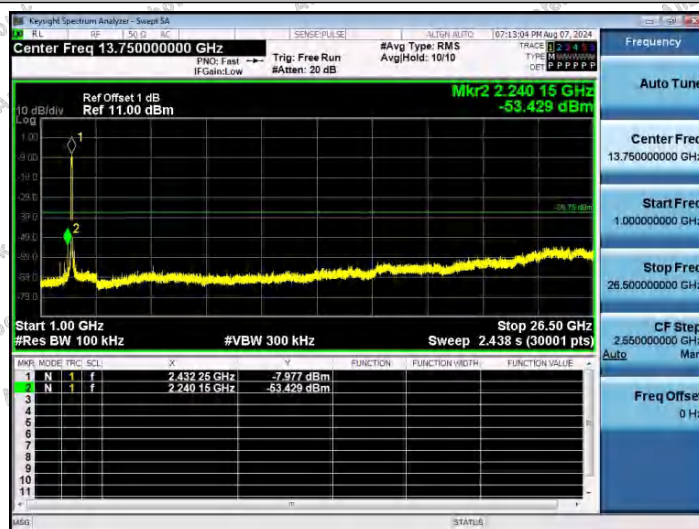
11AX40SISO-Ant1-2437-1000~26500-PASS
