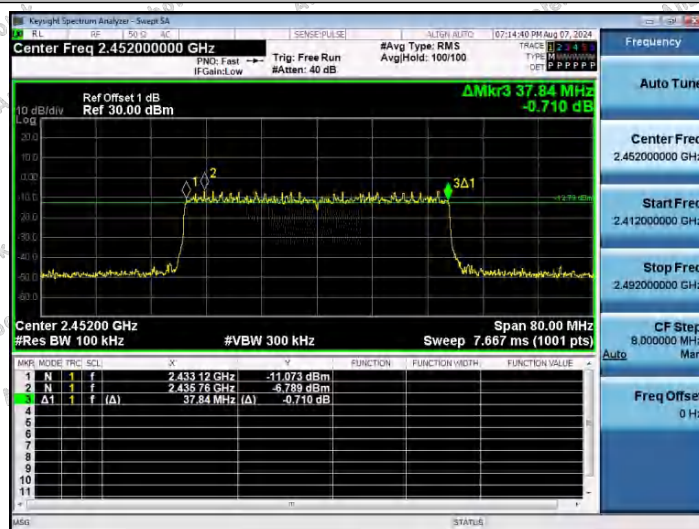
11AX40SISO-Ant1-2452-PASS
