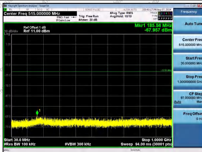
11B-Ant1-2412-30~1000-PASS
