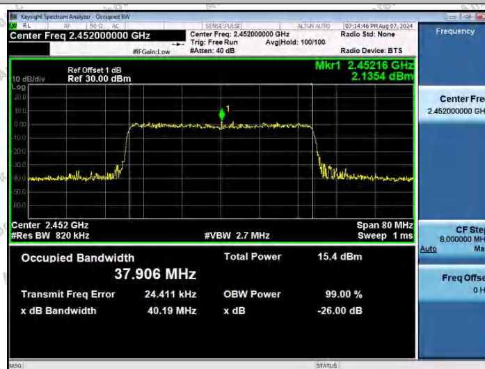
11AX40SISO-Ant1-2452
