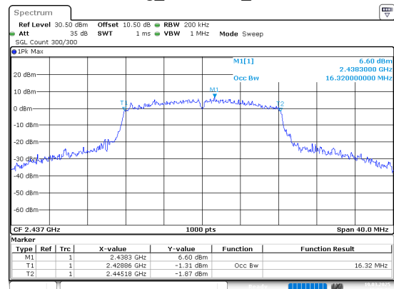
802.11g_2437MHz_Chain 0
