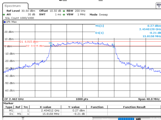
802.11g_2462MHz_Chain 0
