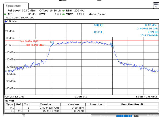
802.11g_2412MHz_Chain 1
