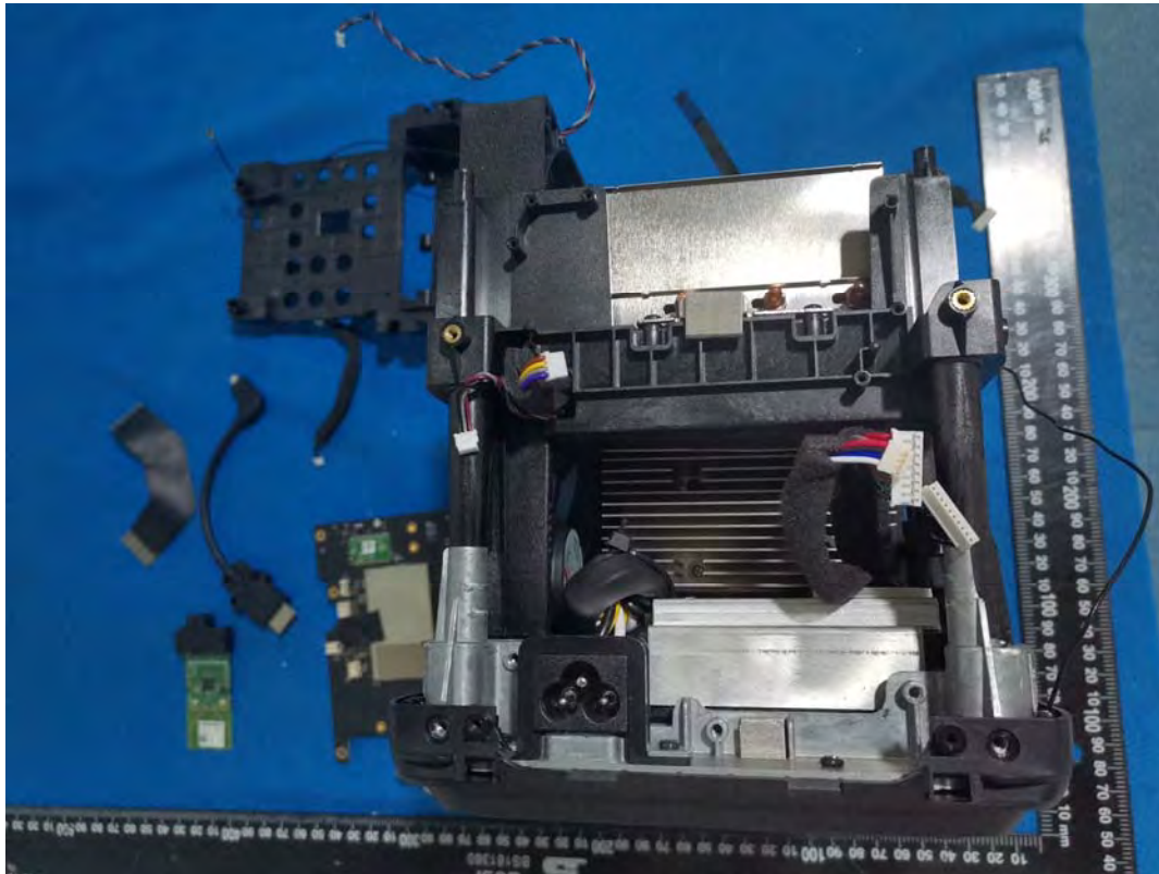
MIC Receiver(SRD) Module
