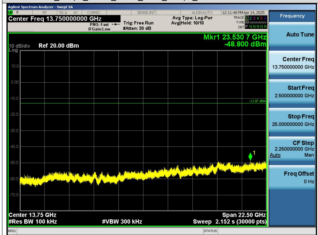
Test_Graph_GFSK_ANT1_2480_2Mbps_Higher Band Emissions
