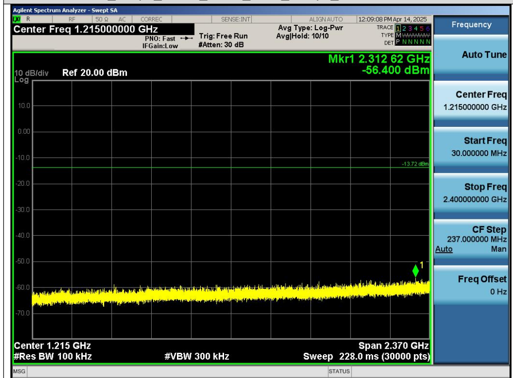
Test_Graph_GFSK_ANT1_2440_2Mbps_Lower Band Emissions
