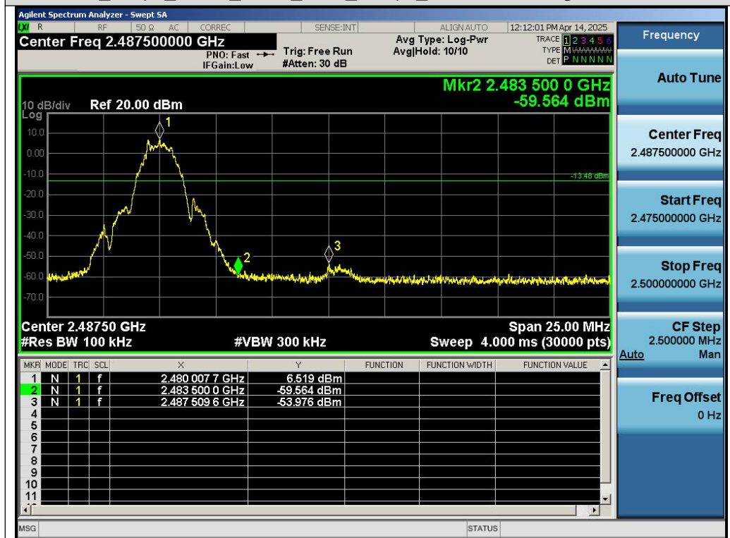
Test_Graph_GFSK_ANT1_2480_2Mbps_Higher Band Edge Emissions
