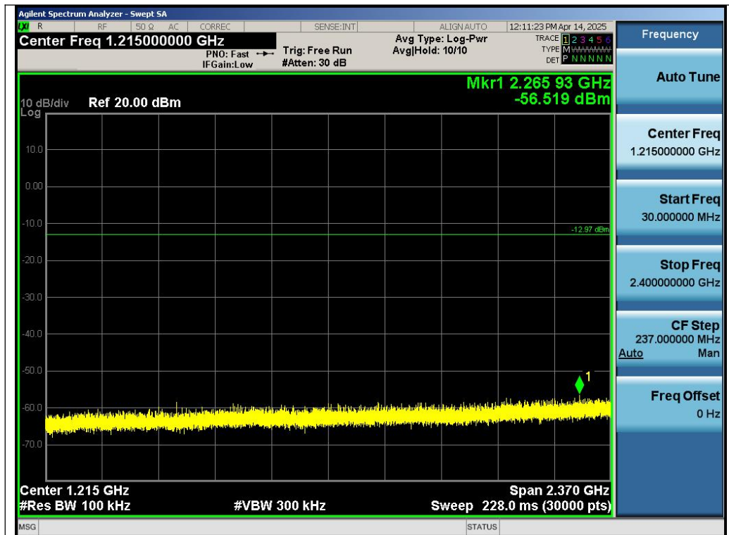
Test_Graph_GFSK_ANT1_2480_2Mbps_Lower Band Emissions
