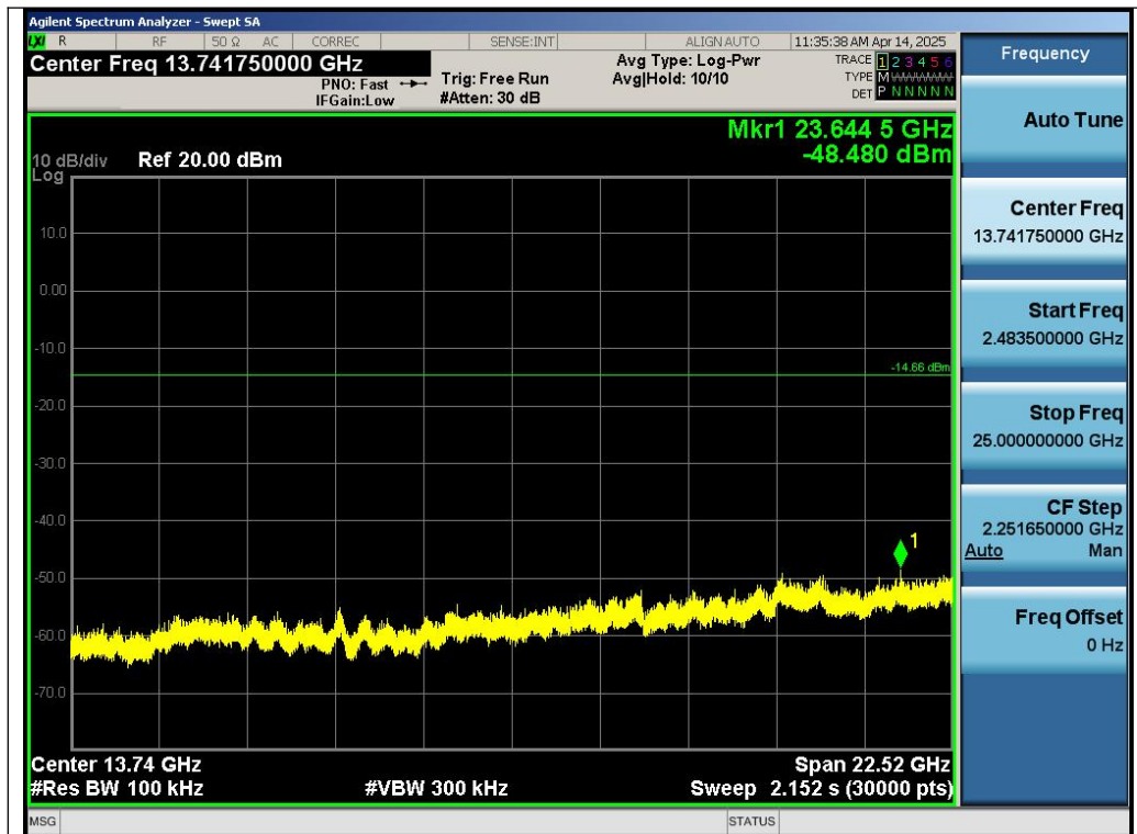
Test_Graph_GFSK_ANT1_2402_1Mbps_Higher Band Emissions
