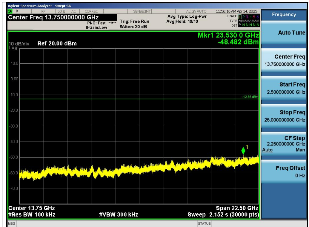
Test_Graph_GFSK_ANT1_2480_1Mbps_Higher Band Emissions
