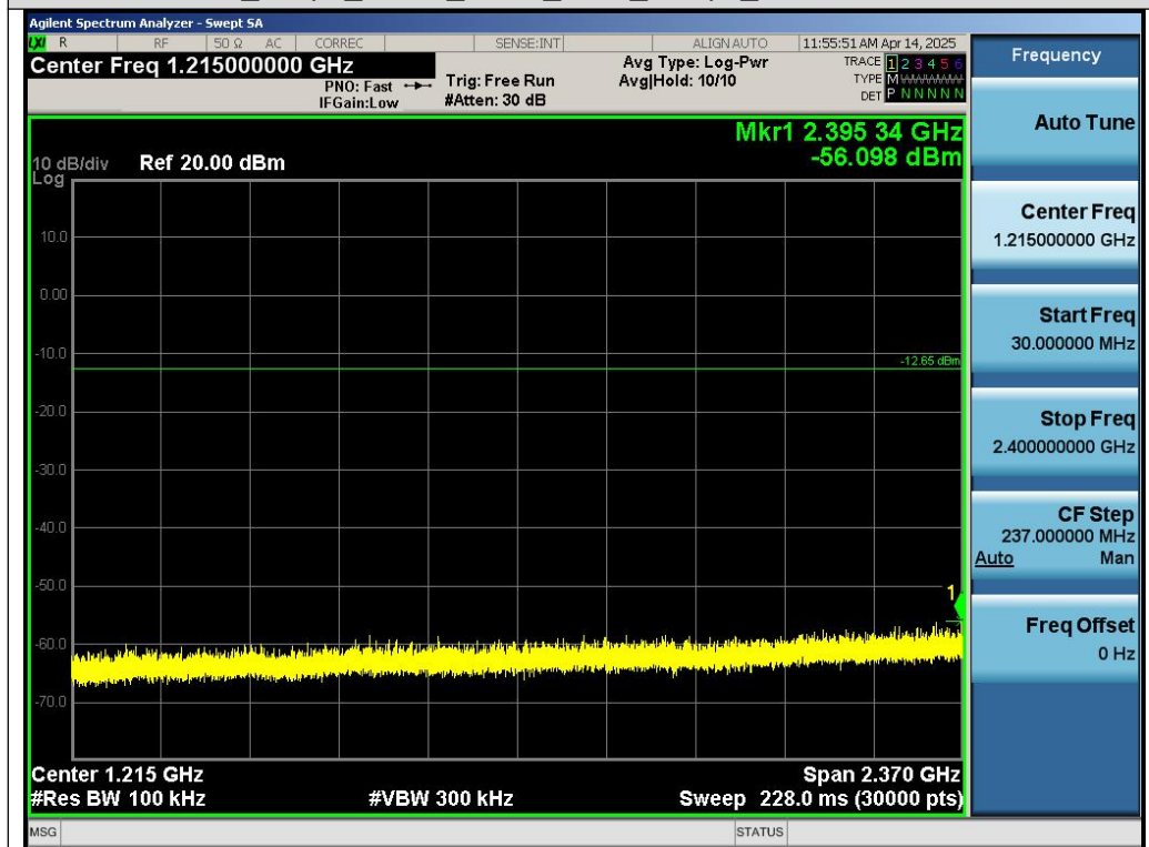
Test_Graph_GFSK_ANT1_2480_1Mbps_Lower Band Emissions
