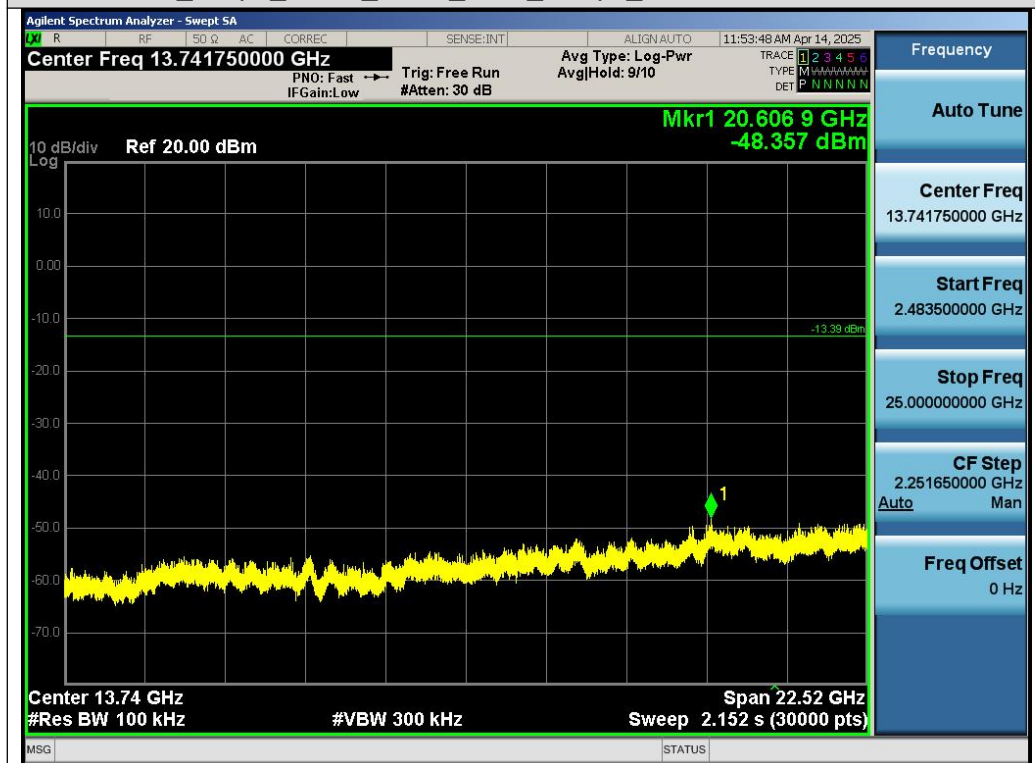
Test_Graph_GFSK_ANT1_2440_1Mbps_Higher Band Emissions
