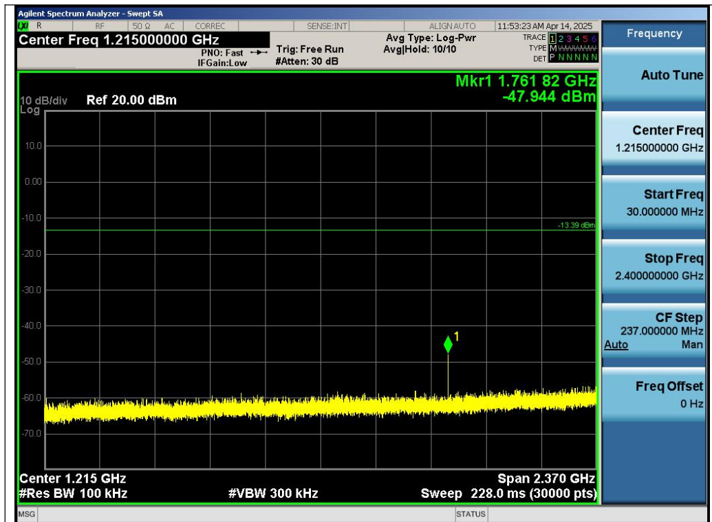
Test_Graph_GFSK_ANT1_2440_1Mbps_Lower Band Emissions
