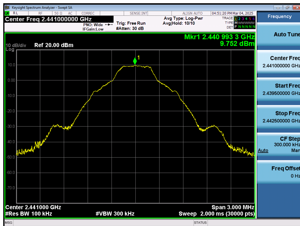
Test_Graph_BR_ANT1_2441_1Mbps_Reference Level
