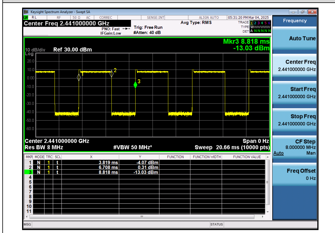
EDR-8DPSK-ANT1-2441
