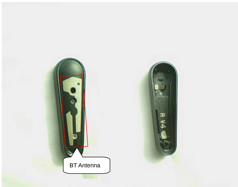
ANTENNA CLOSE-UP PHOTO-1
