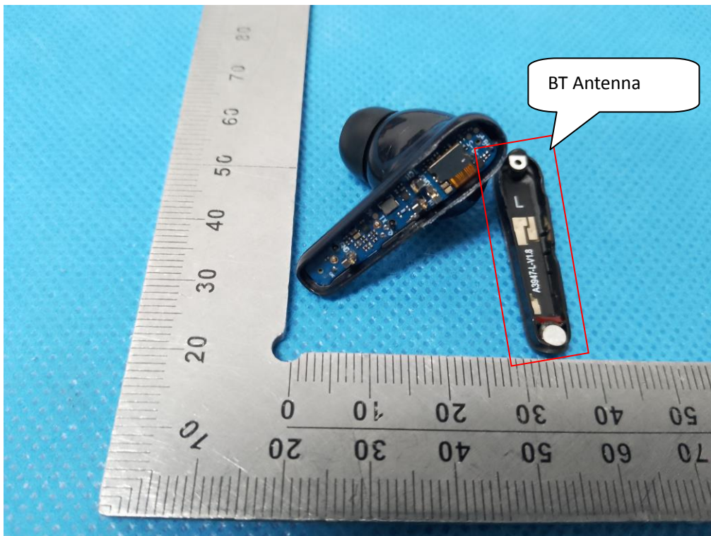
OPEN VIEW OF EUT (FIGURE 1) (Left)
