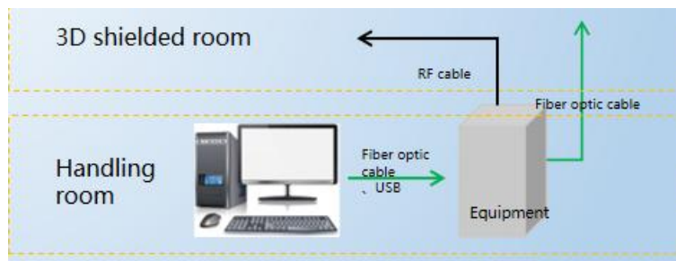
Picture1.Antenna static test connection method
