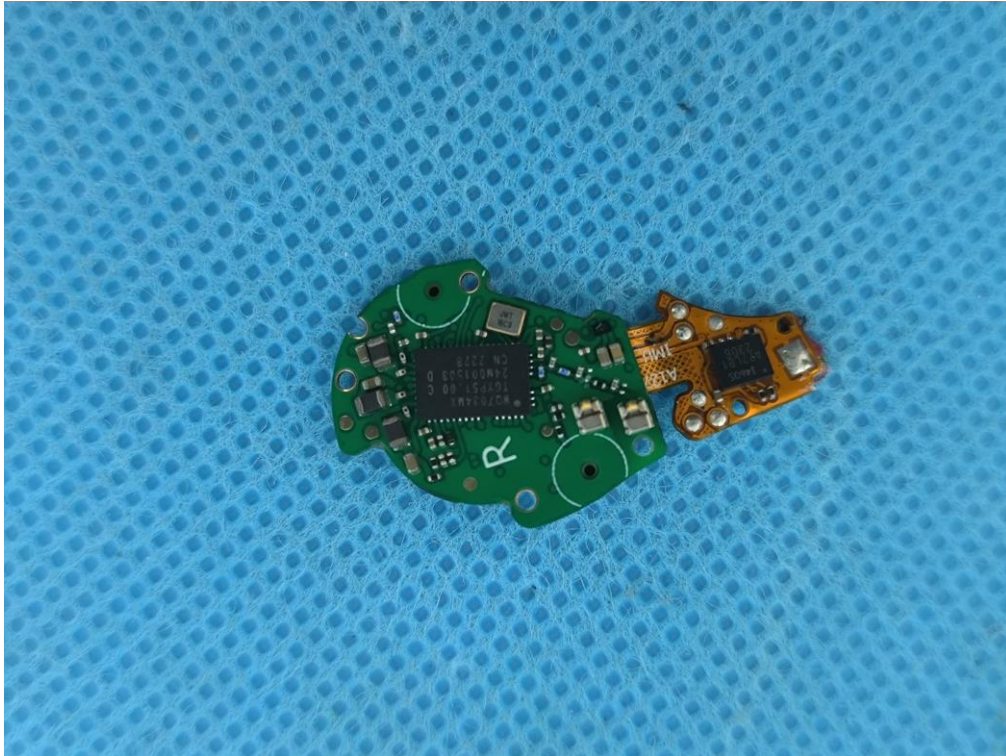
OPEN VIEW OF EUT (FIGURE 1) –WITH BATTERY HT78250VS
