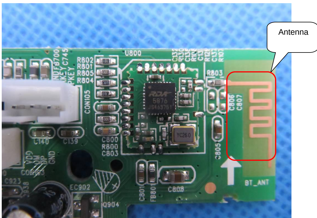
INTERNAL VIEW OF EUT-10
