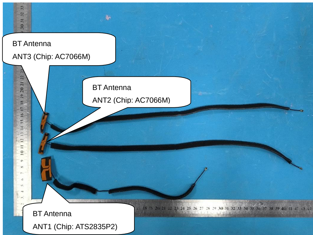
ANTENNA CLOSE-UP PHOTO-5
