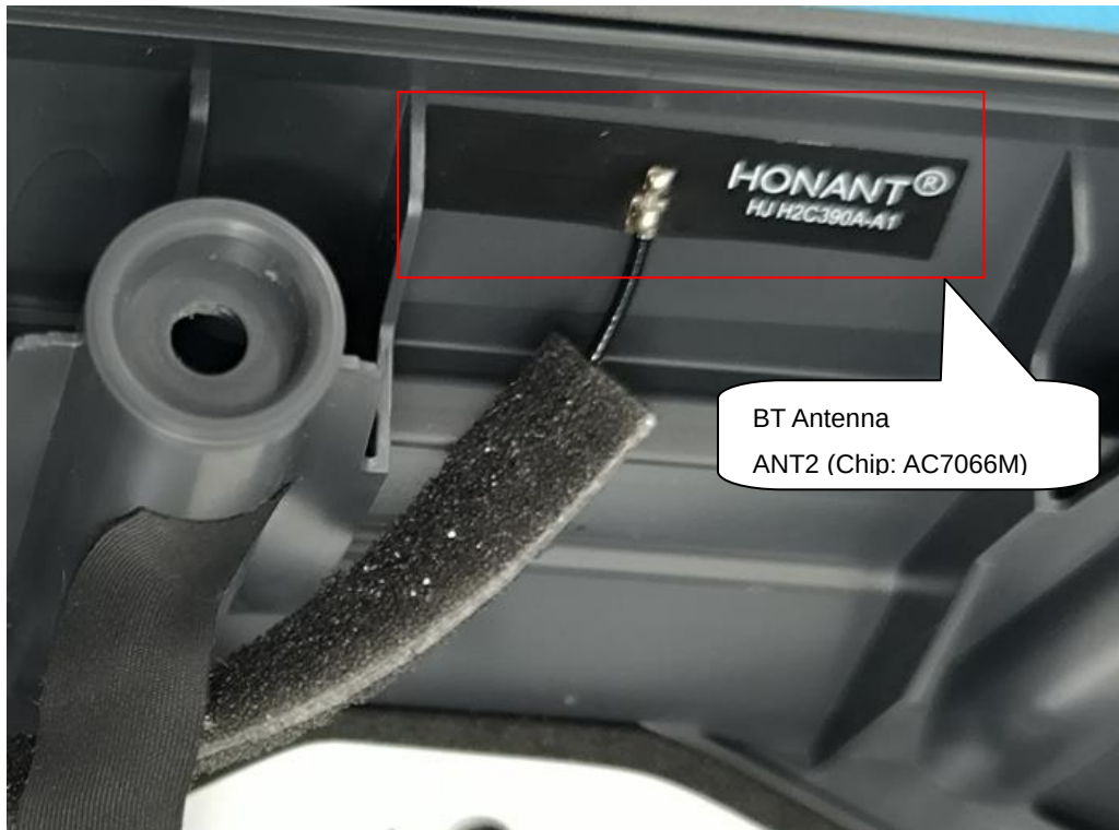
ANTENNA CLOSE-UP PHOTO-3
