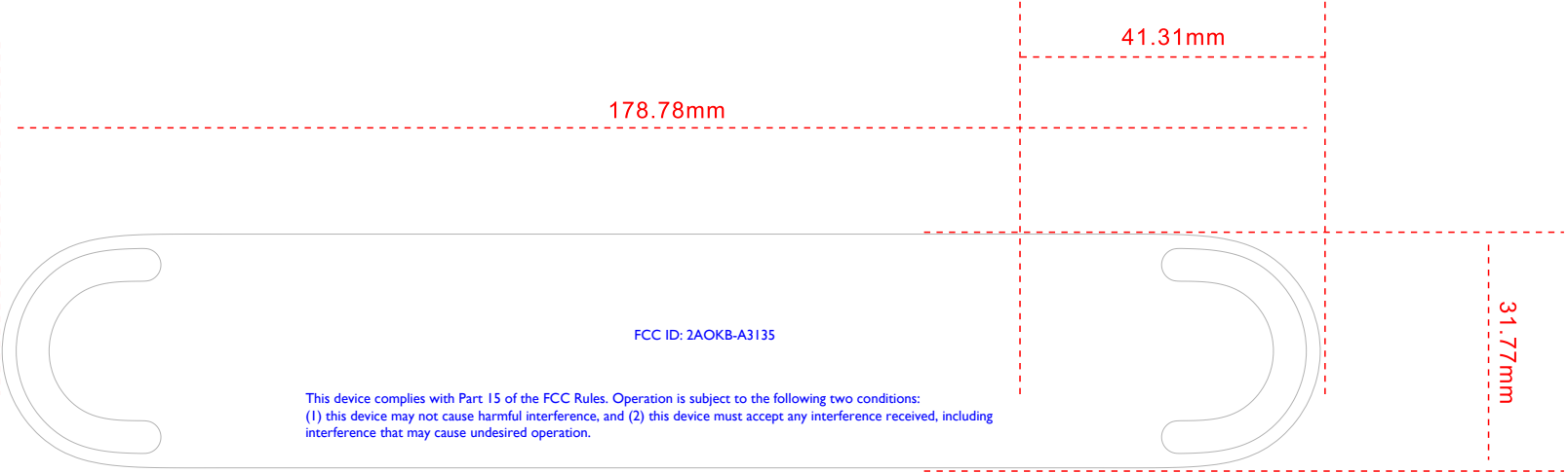
Back view of EUT
