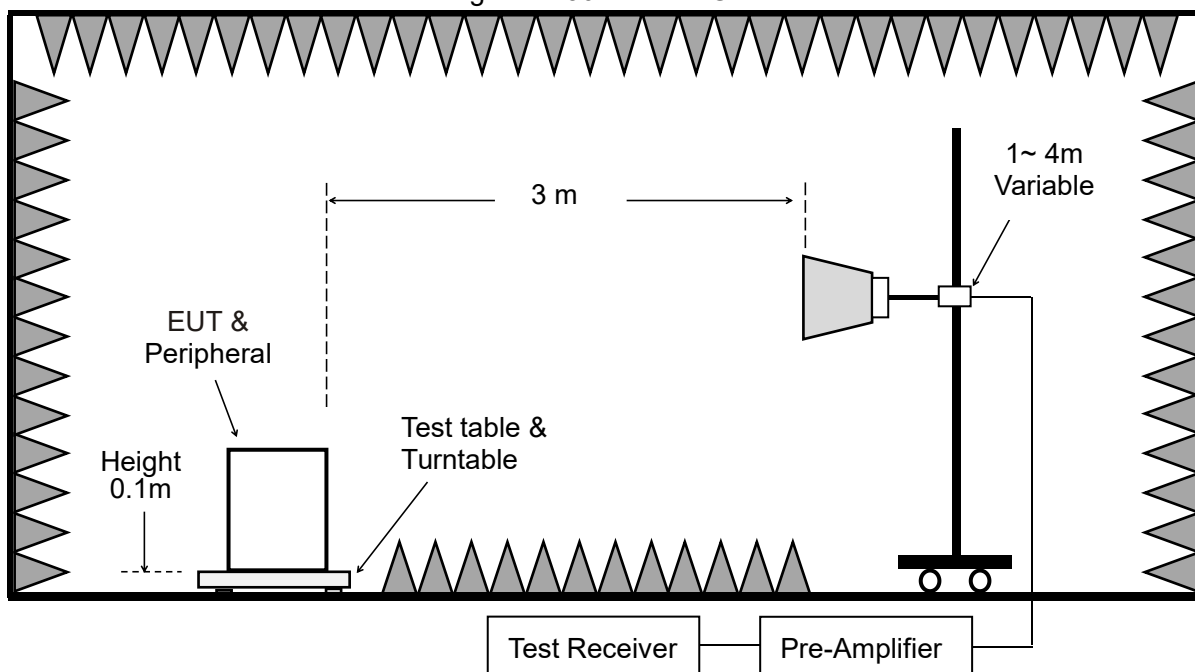
Figure 3. Above 1 GHz
