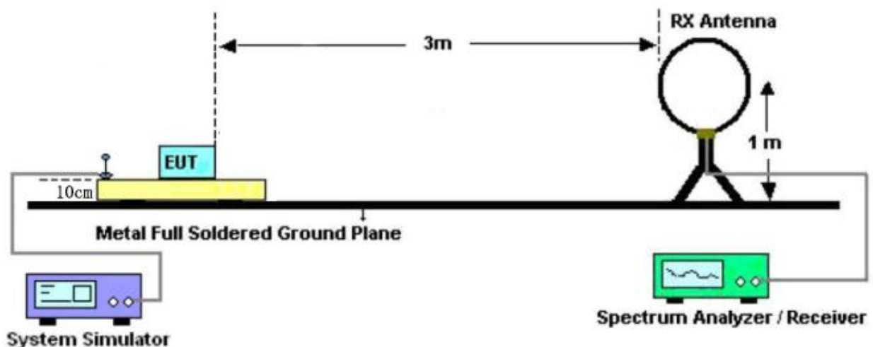
Figure 1. Below 30MHz
