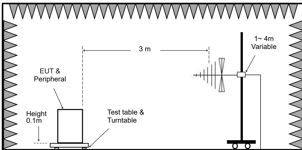
Figure 2. 30MHz to 1GHz
