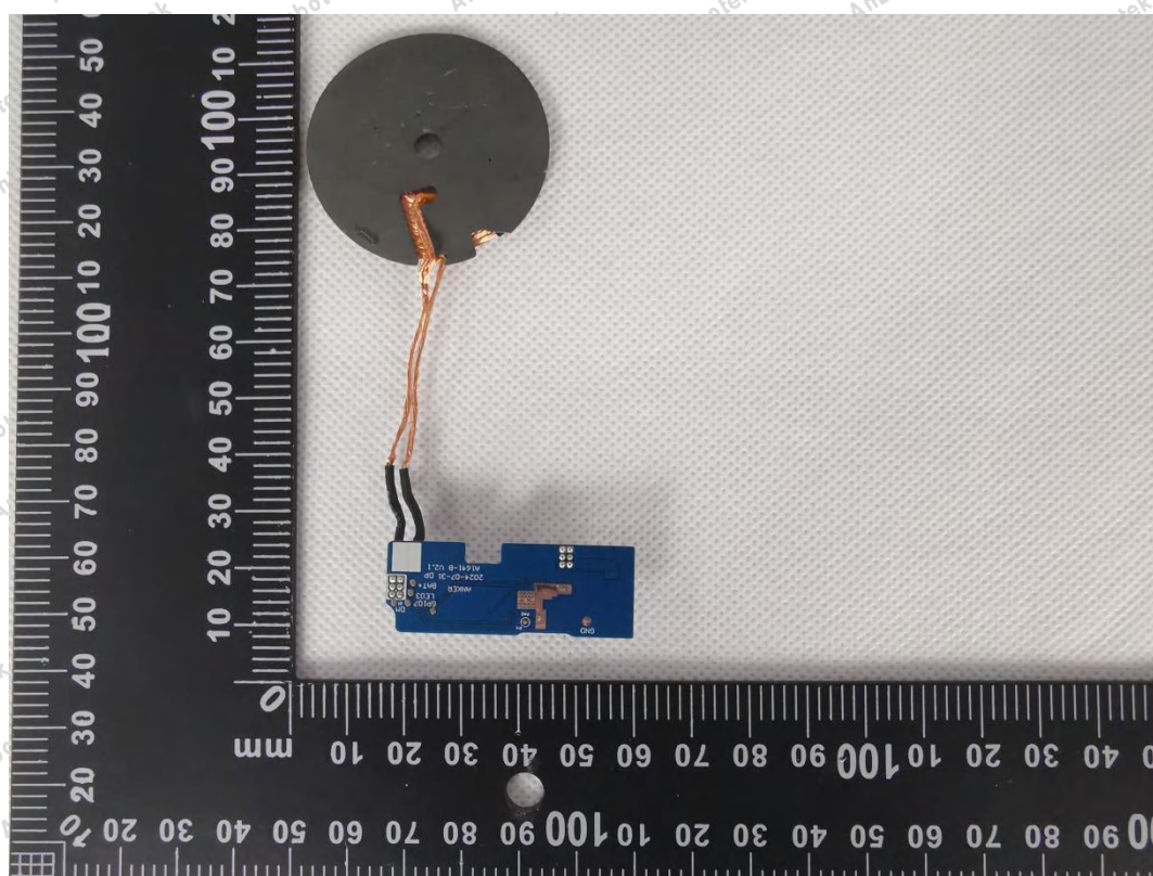
Inductive loop coil Antenna
