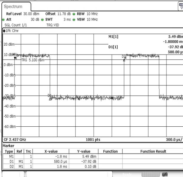
NTNV-11N40SISO-Ant1-2437
