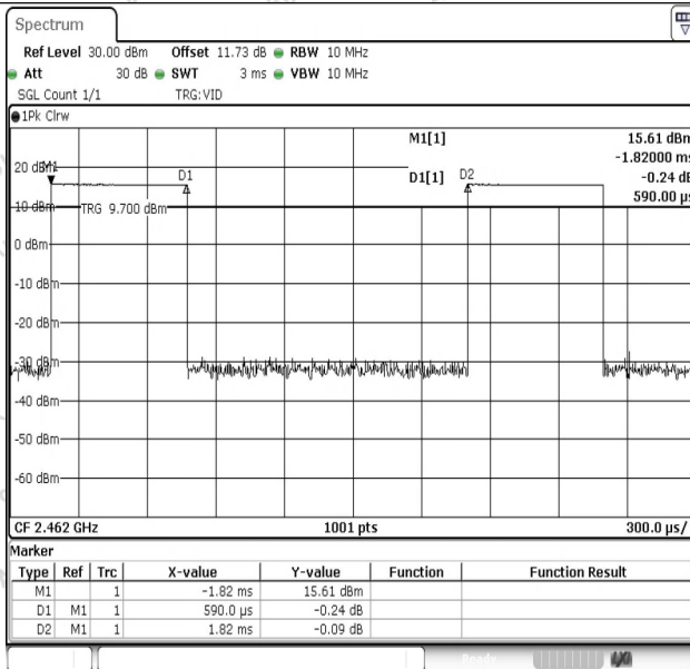
NTNV-11B-Ant1-2462
