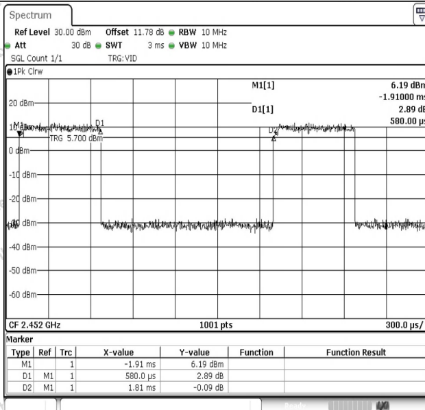
NTNV-11N40SISO-Ant1-2452
