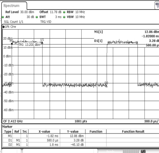
NTNV-11G-Ant1-2412
