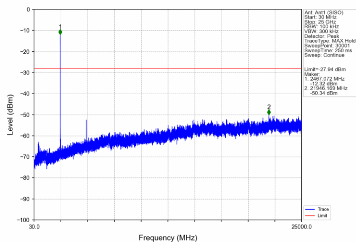
802.11ax(HEW40)_HCH_2452MHz_RU484_65_Ant1 (SISO)_NTNV
