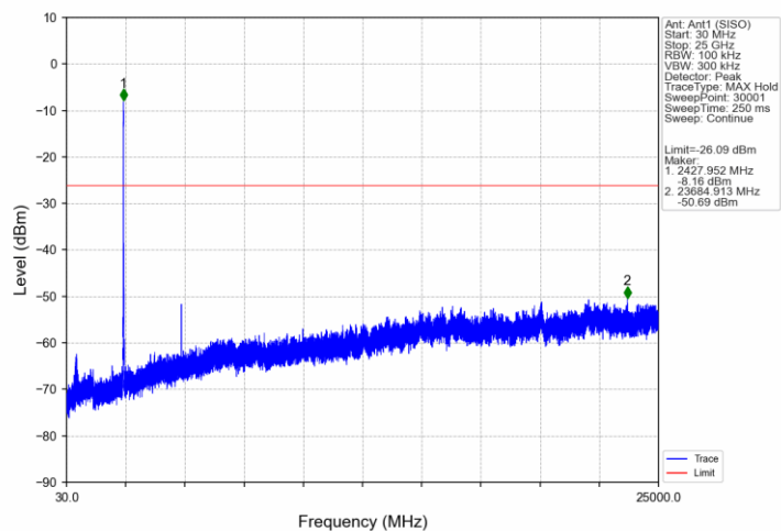
802.11ax(HEW40)_MCH_2437MHz_RU484_65_Ant1 (SISO)_NTNV
