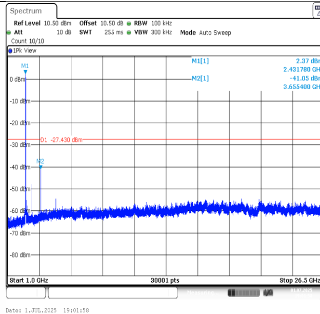
11N20SISO-Ant1-2437-1000-26500-PASS
