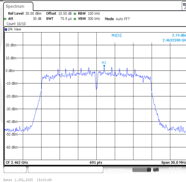
11N20SISO-Ant1-2462-0-Reference-PASS
