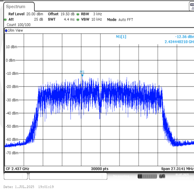
11N20SISO-Ant1-2437-PASS
