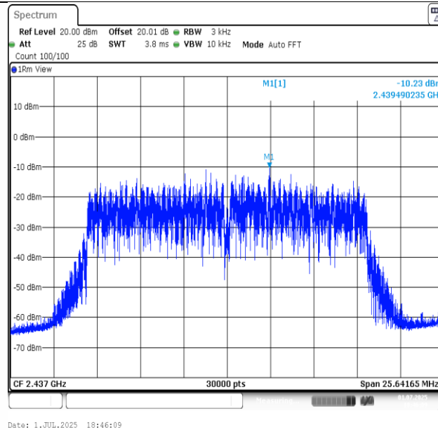
11G-Ant1-2437-PASS
