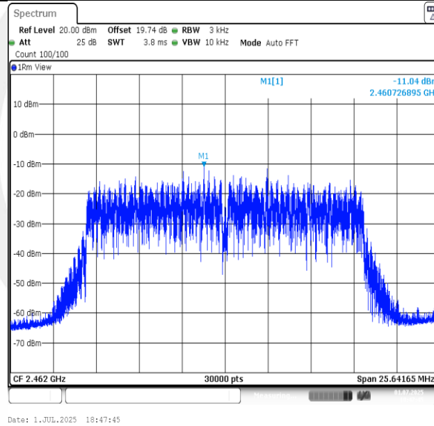
11G-Ant1-2462-PASS
