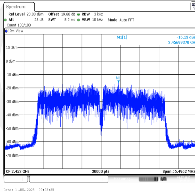
11N40SISO-Ant1-2452-PASS
