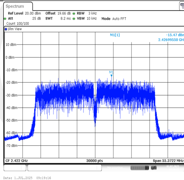
11N40SISO-Ant1-2422-PASS
