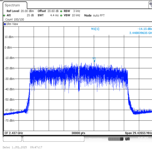
11AX20SISO-Ant1-2437-PASS
