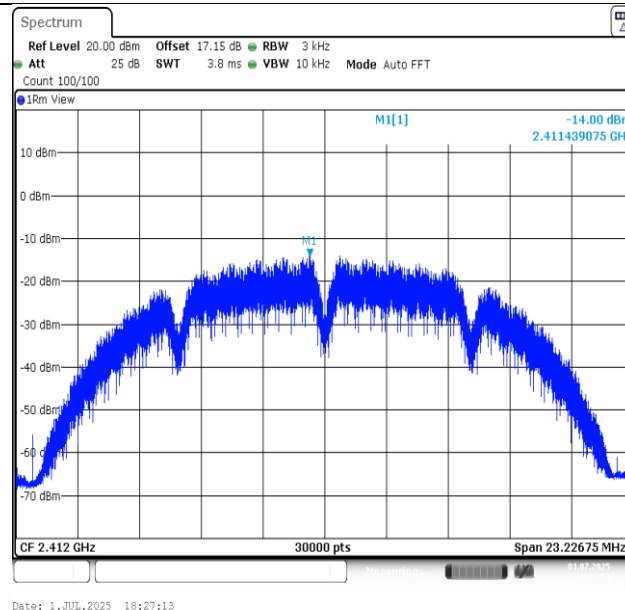
11B-Ant1-2412-PASS
