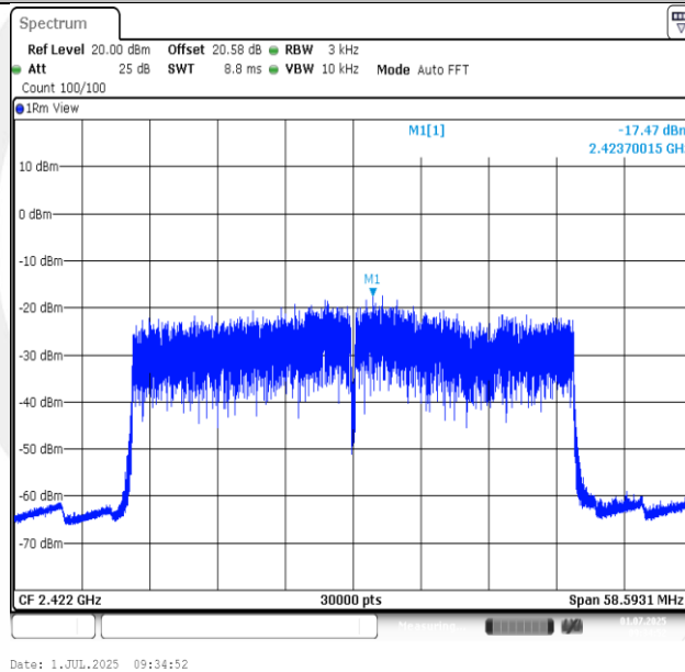
11AX40SISO-Ant1-2422-PASS
