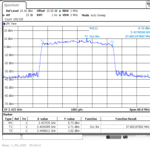
11AX40SISO-Ant1-2422
