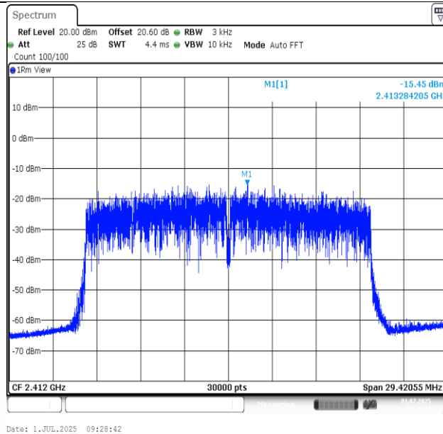
11AX20SISO-Ant1-2412-PASS
