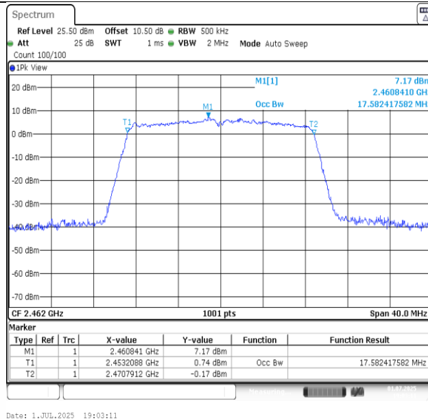
11N20SISO-Ant1-2462
