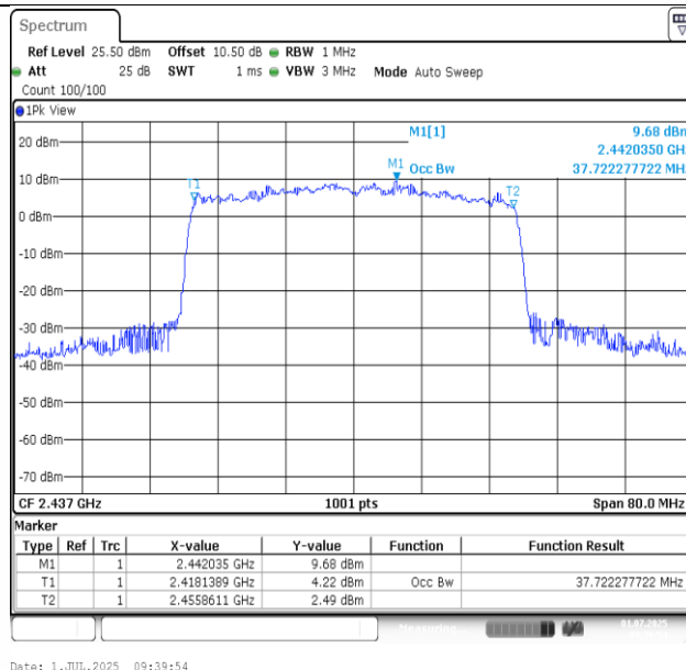
11AX40SISO-Ant1-2437
