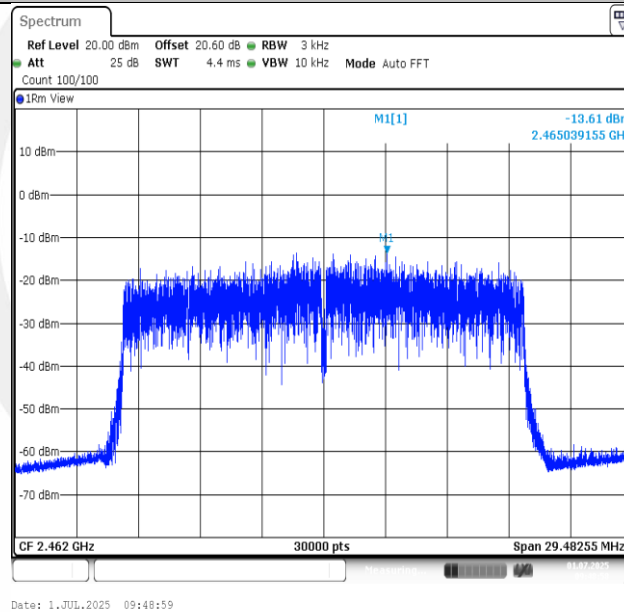
11AX20SISO-Ant1-2462-PASS
