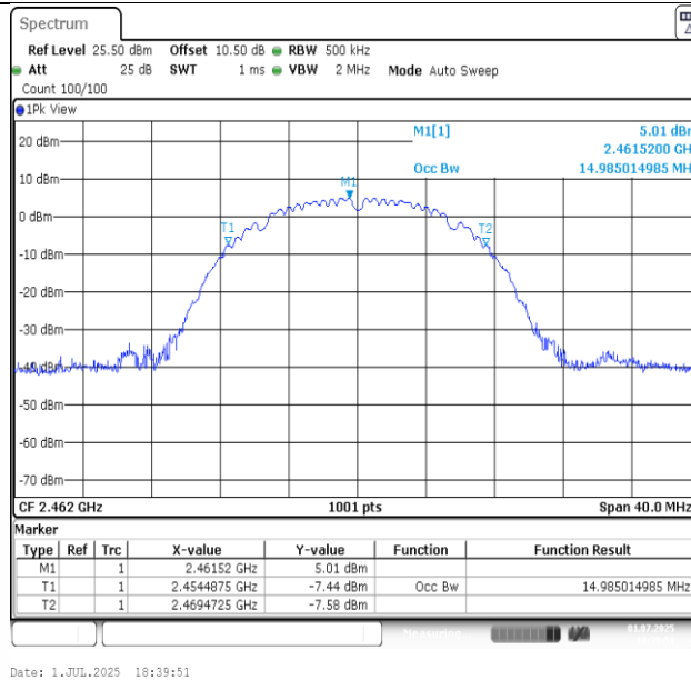
11B-Ant1-2462
