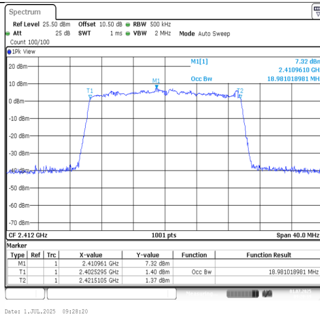
11AX20SISO-Ant1-2412
