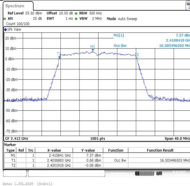
11G-Ant1-2412
