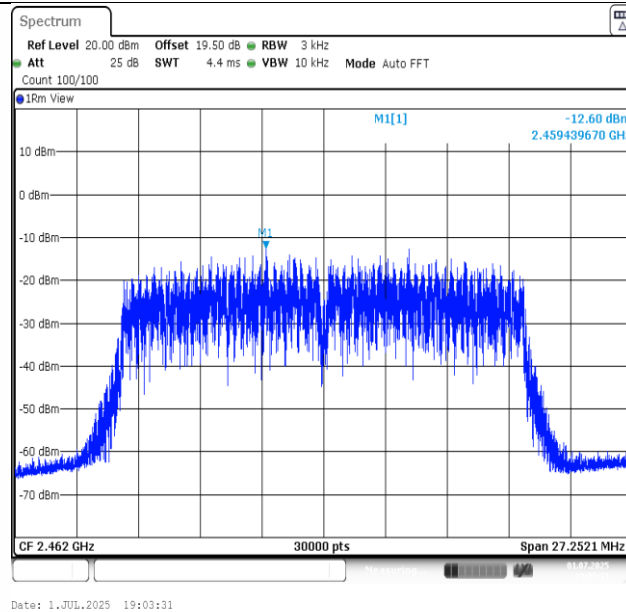
11N20SISO-Ant1-2462-PASS
