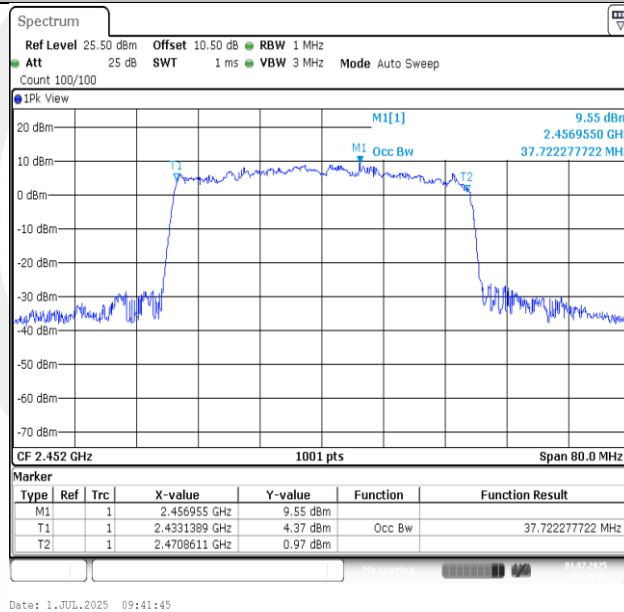
11AX40SISO-Ant1-2452
