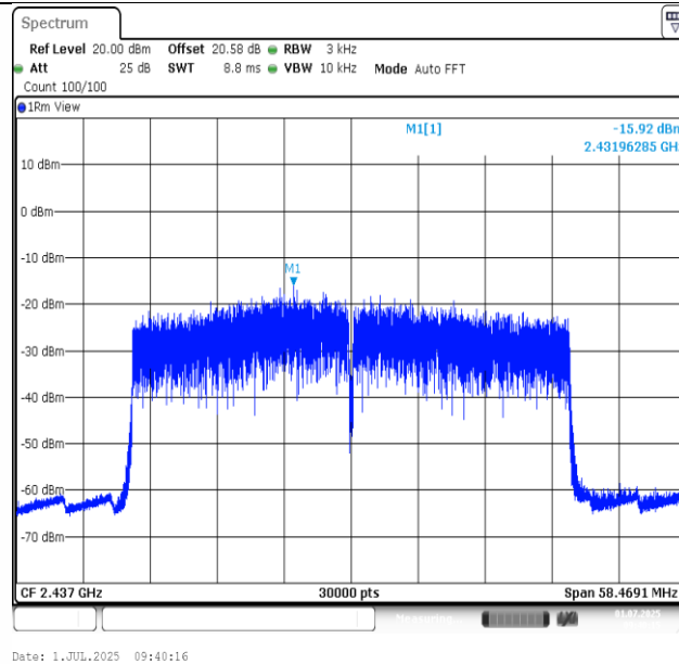
11AX40SISO-Ant1-2437-PASS
