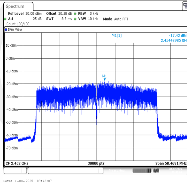
11AX40SISO-Ant1-2452-PASS
