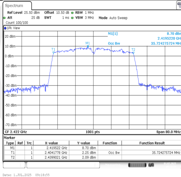
11N40SISO-Ant1-2422
