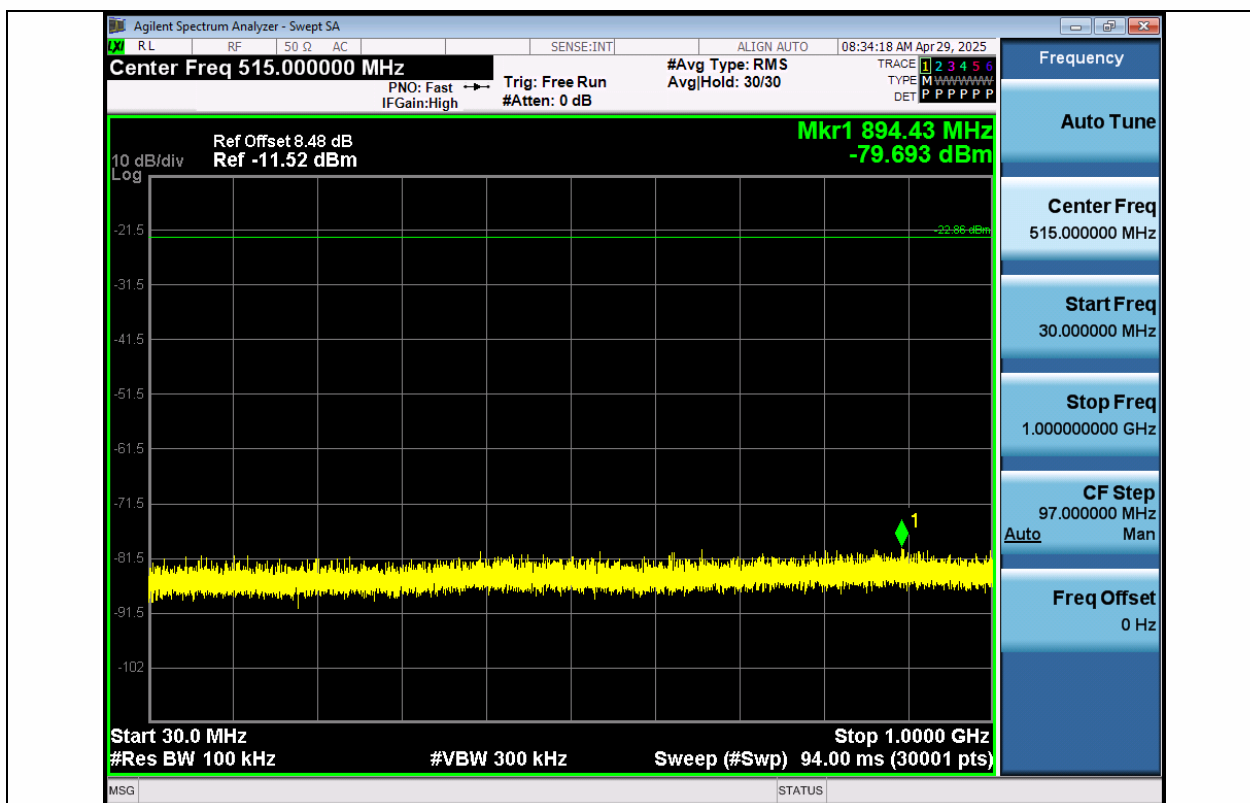
BLE_1M-Ant1-2402-30~1000-PASS
