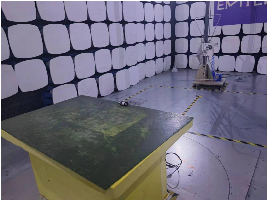
Photos of Radiation Emission Measurement
