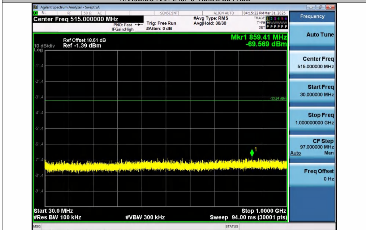
11N40SISO-Ant1-2437-30~1000-PASS
