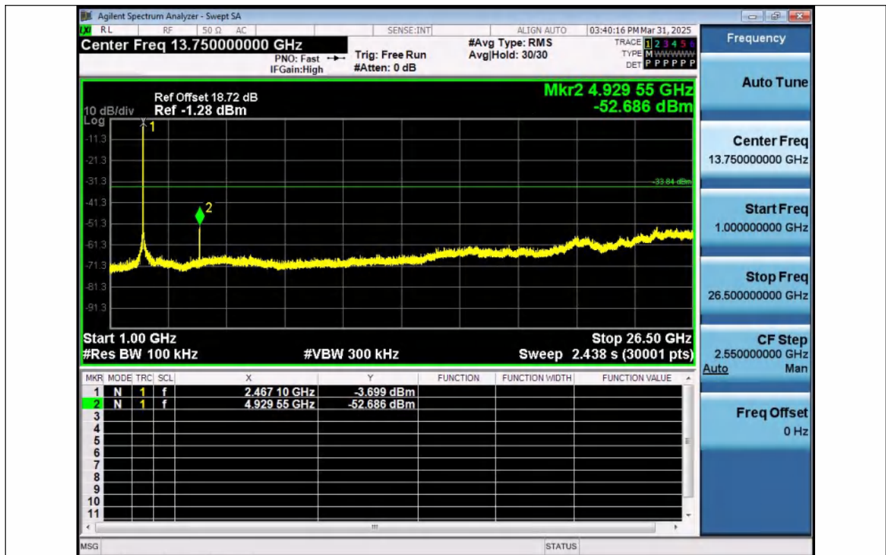
11N20SISO-Ant1-2462-1000~26500-PASS
