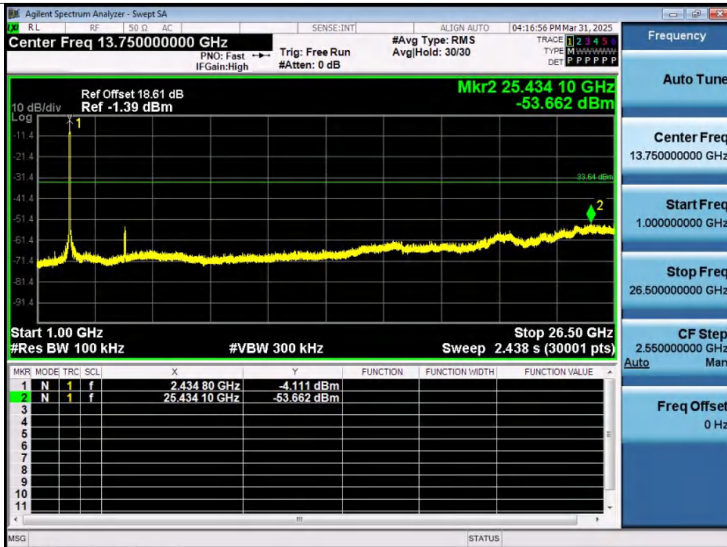
11N40SISO-Ant1-2437-1000~26500-PASS
