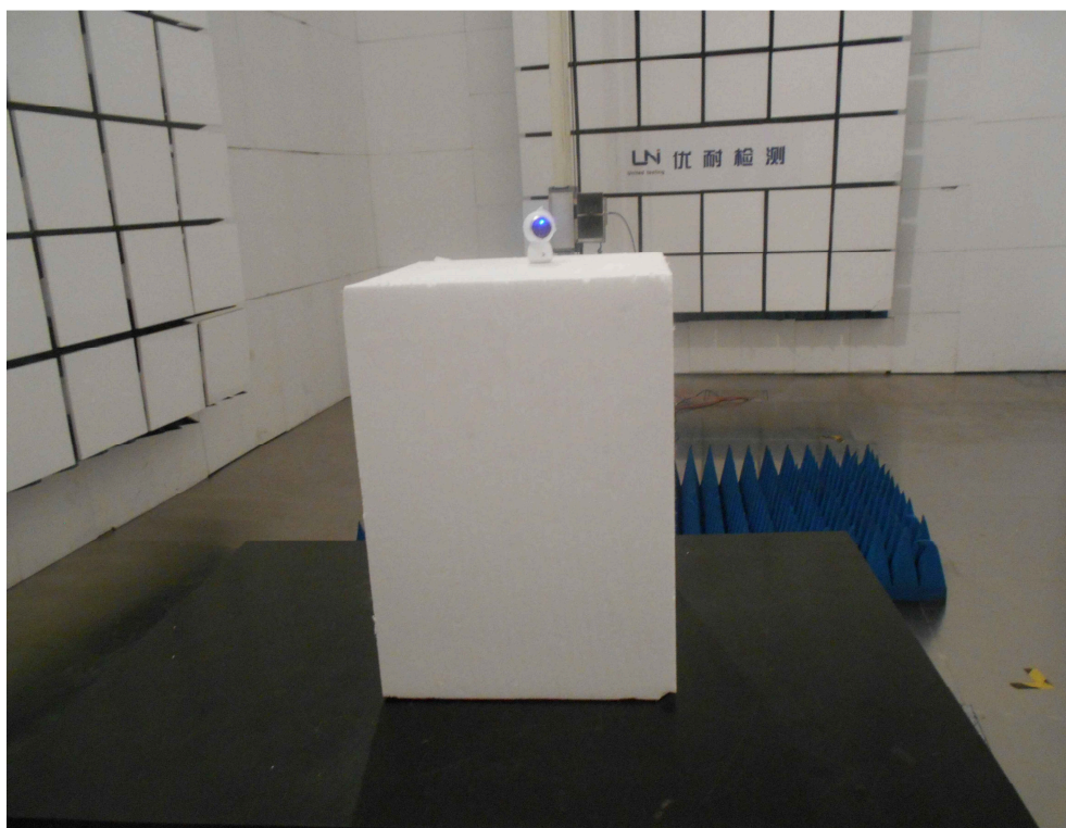
Radiated Emission (Above 1G)
