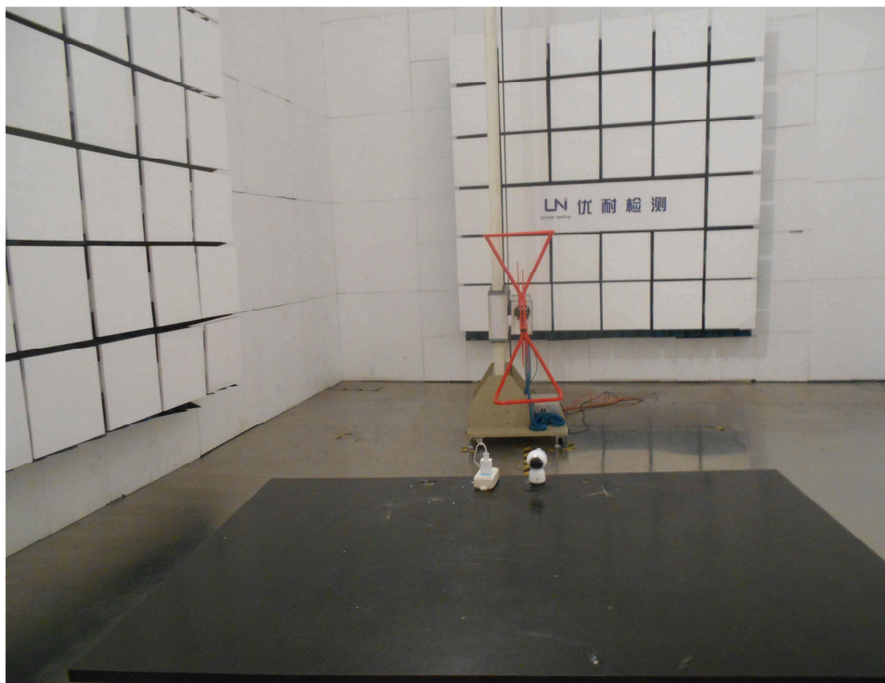
Radiated Emission (Below 1G)
