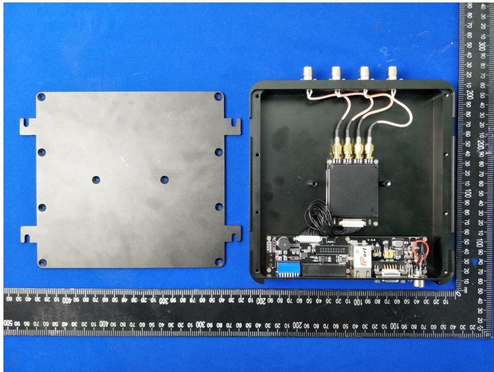
2dBi Antenna Interior Photos
