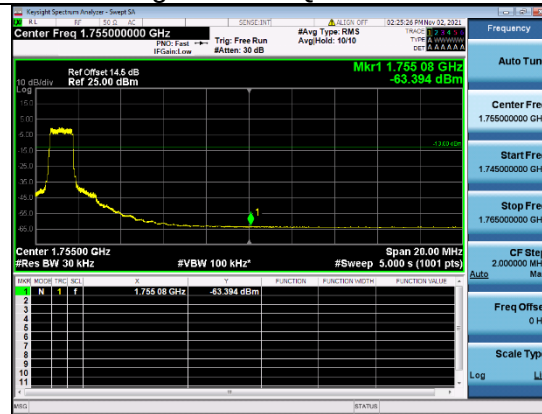
B4-10M-High CH-CSE-1-QPSK-1 RB 0
