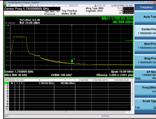
B4-5M-High CH-CSE-1-QPSK-1 RB 0
