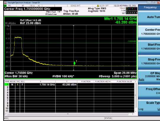
B4-10M-High CH-BE-QPSK-Full RB 0
