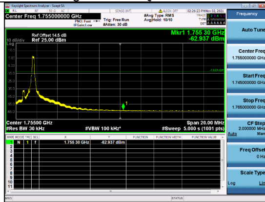
B4-10M-High CH-CSE-1-Q16-1 RB 0
