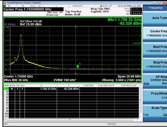
B4-10M-High CH-BE-QPSK-1 RB MAX
