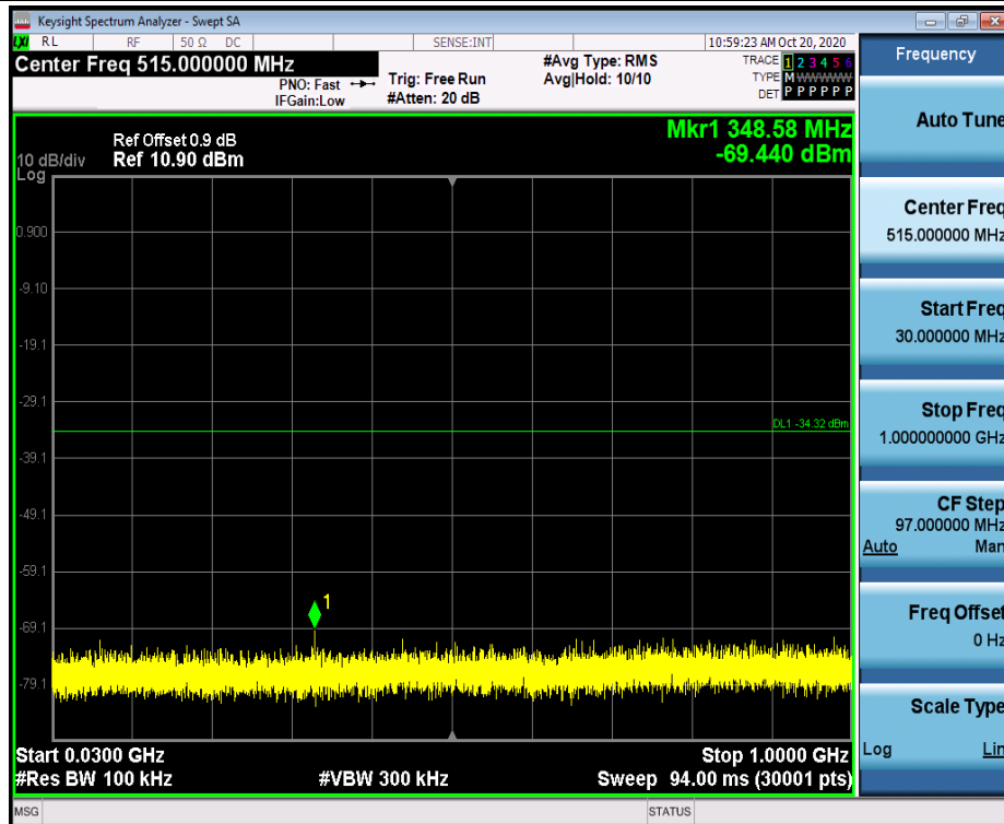
BLE_1M_Ant1_2440_30~1000
