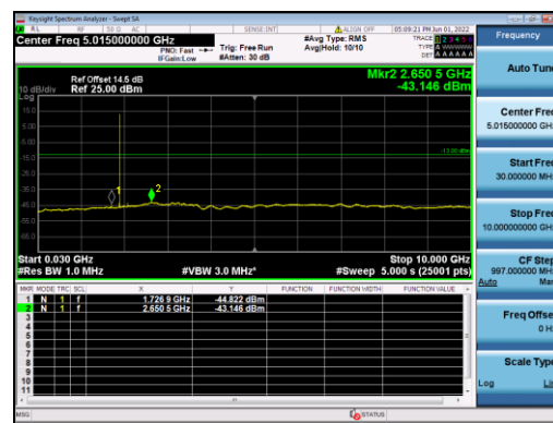
B2-5M-High CH-CSE-2-QPSK-1 RB 0
