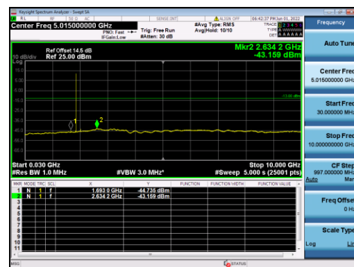
B4-1.4M-High CH-CSE-2-Q16-1 RB 0
