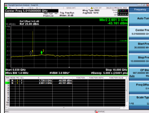
B2-15M-High CH-CSE-1-QPSK-1 RB 0
