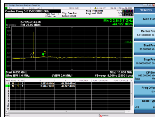
B4-1.4M-High CH-CSE-2-QPSK-1 RB 0
