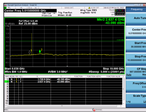
B2-3M-High CH-CSE-2-QPSK-1 RB 0
