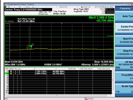
B2-20M-High CH-CSE-2-QPSK-1 RB 0
