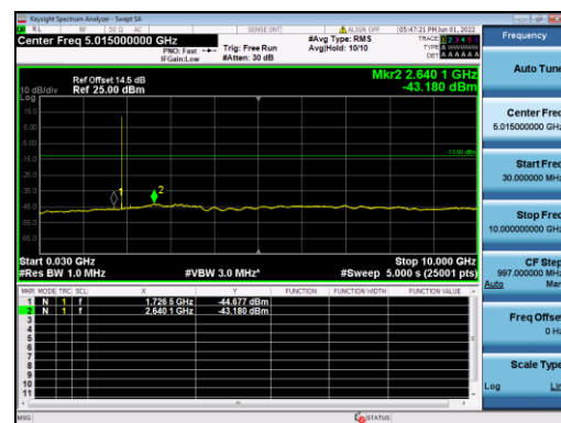
B2-10M-High CH-CSE-1-QPSK-1 RB 0
