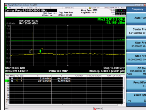
B2-1.4M-High CH-CSE-2-QPSK-1 RB 0
