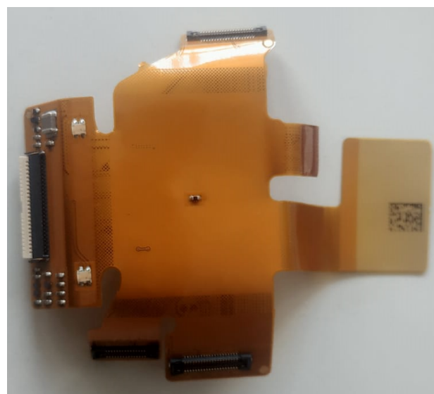
Figure 6: Bottom View, ScanFlex PCB
