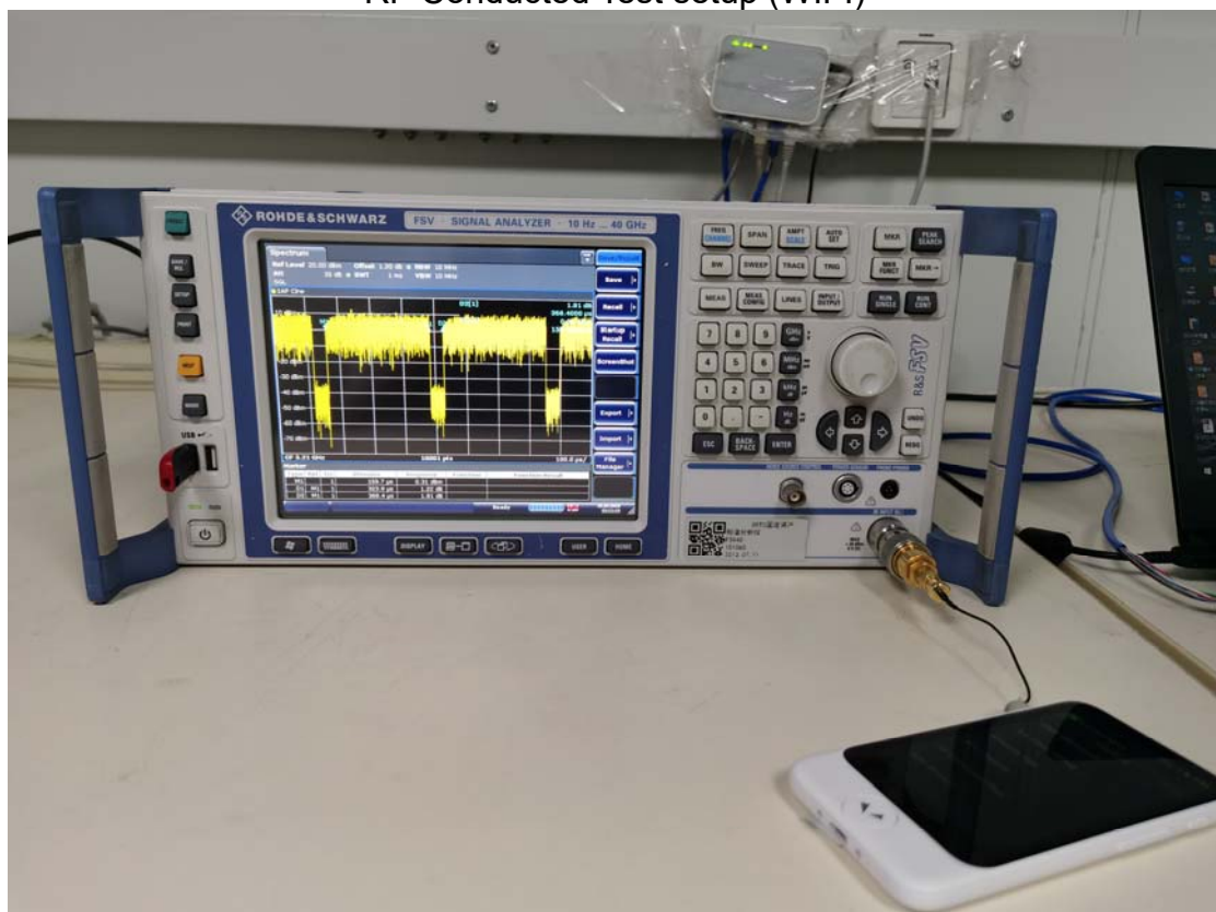
RF Conducted Test setup (BT/BLE)
