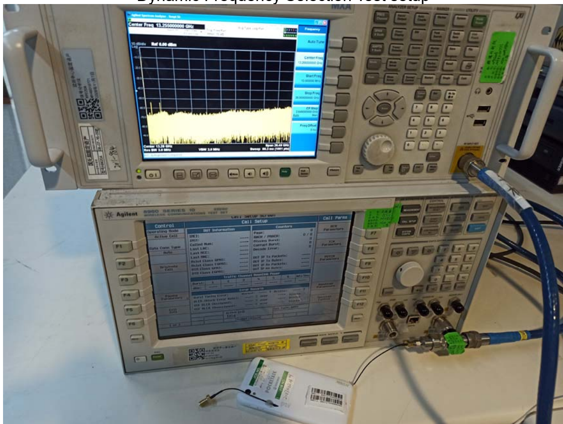
RF Conducted Test setup (GSM/WCDMA)
