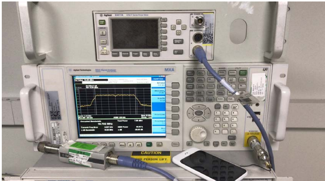
RF Conducted Test setup (WIFI)
