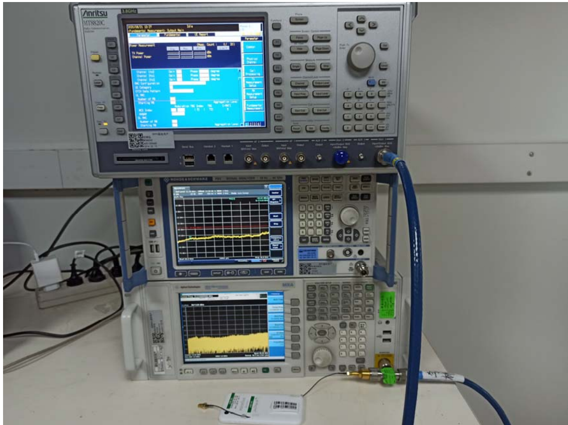
RF Conducted Test setup (LTE)
