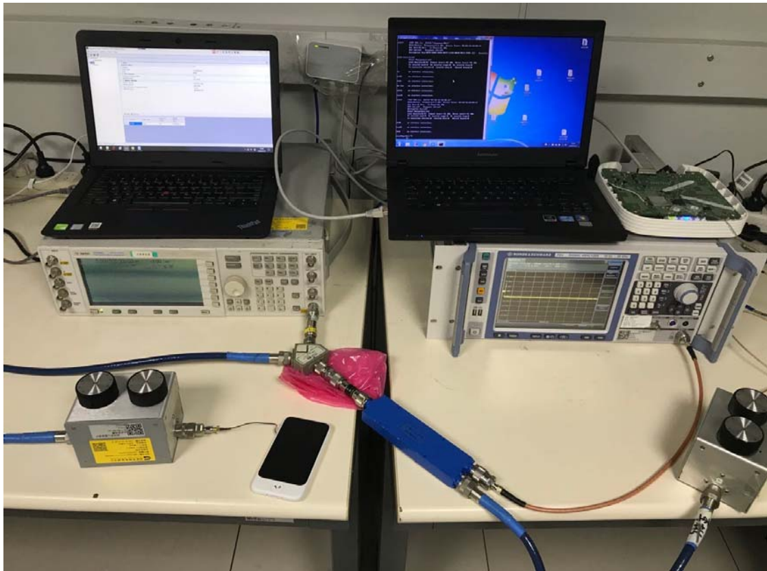
Dynamic Frequency Selection Test setup
