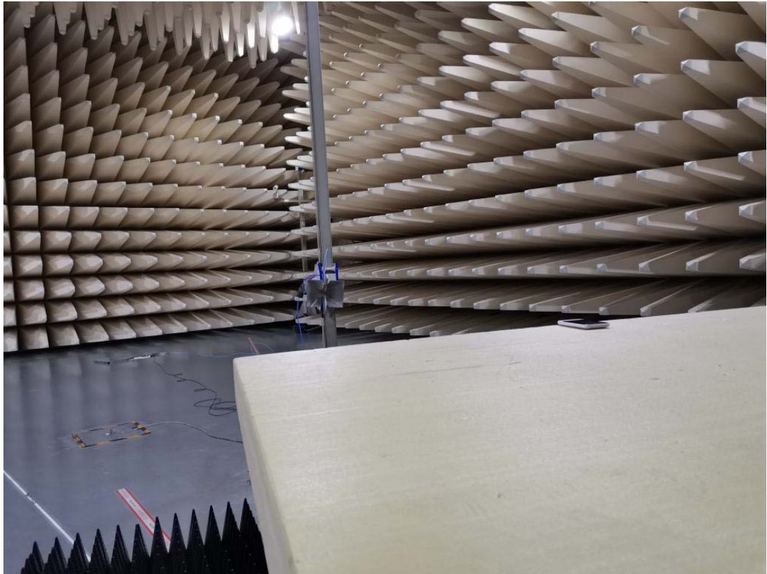
Spurious Radiated Emissions Test setup
