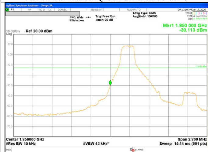
LTE Band 2 1.4MHz QPSK Low Channel RB6-0
