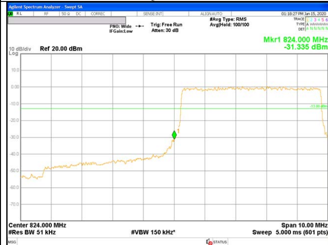
LTE Band 5 5MHz QPSK Low Channel RB25-0
