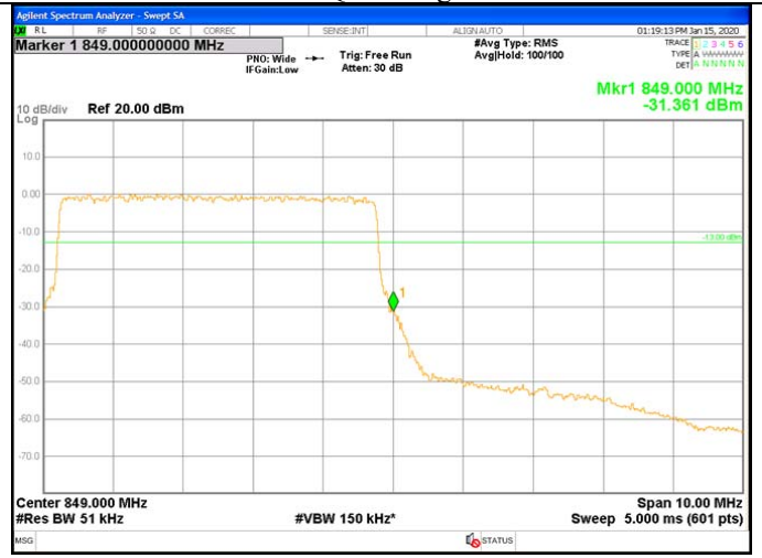
LTE Band 5 5MHz QPSK High Channel RB25-0
