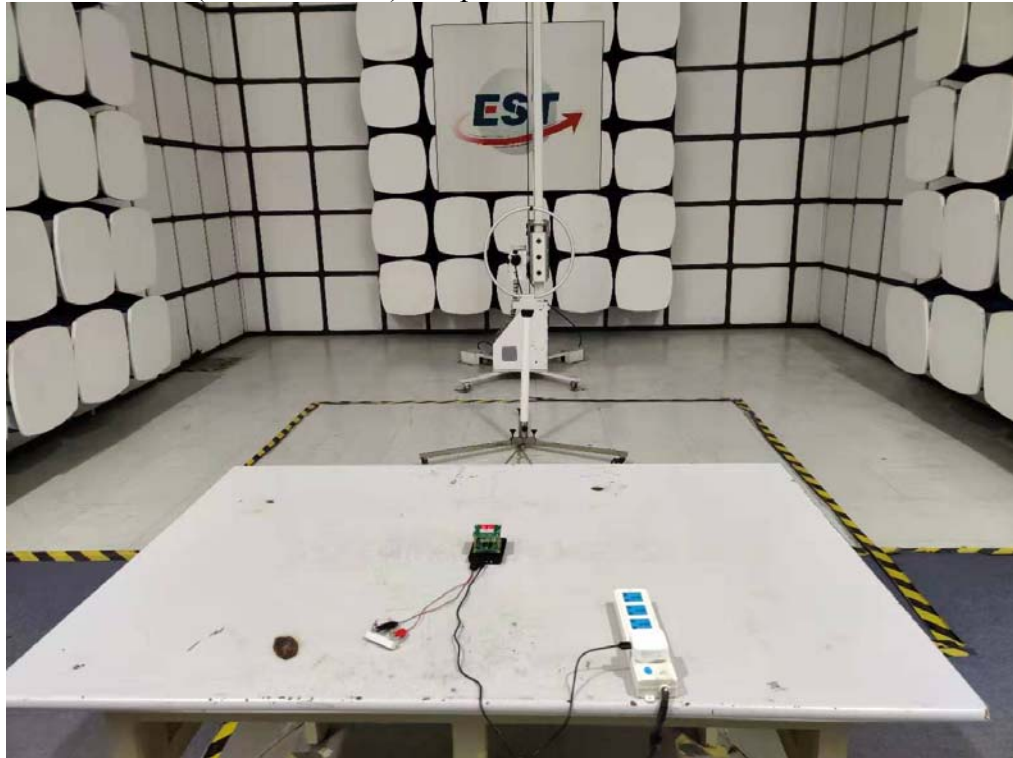
Radiated Test (9kHz-30 MHz) Adapter
