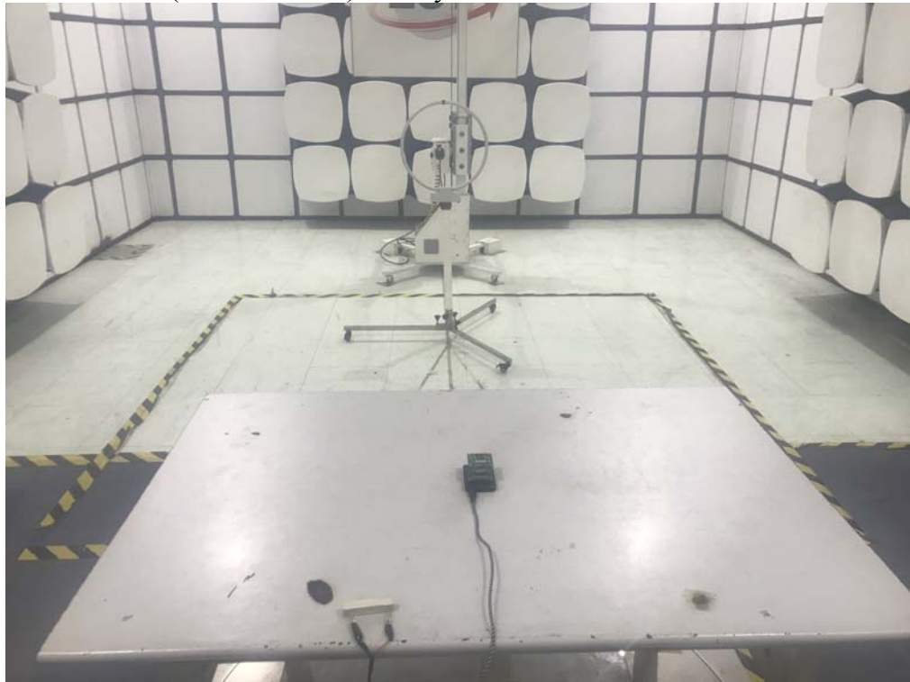
Radiated Test (9kHz-30 MHz) Battery
