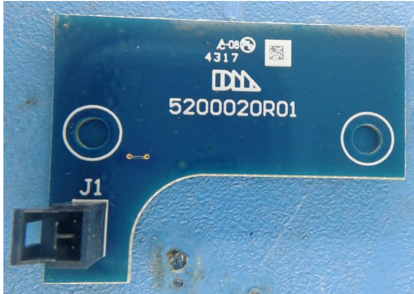
View of top side of antenna PCBA
