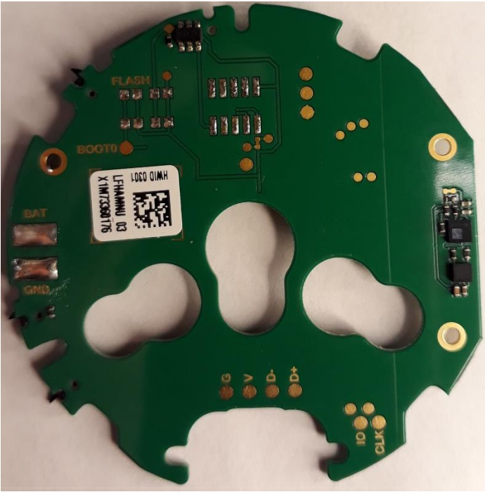
PCB backside
