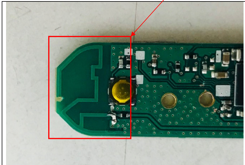
PCB Patten Antenna
