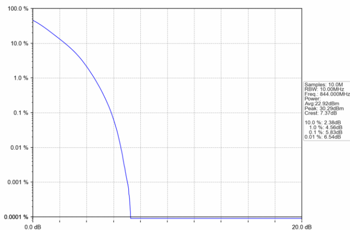
Band5 10MHz QPSK HCH 844MHz RB 50 0 NTNV
