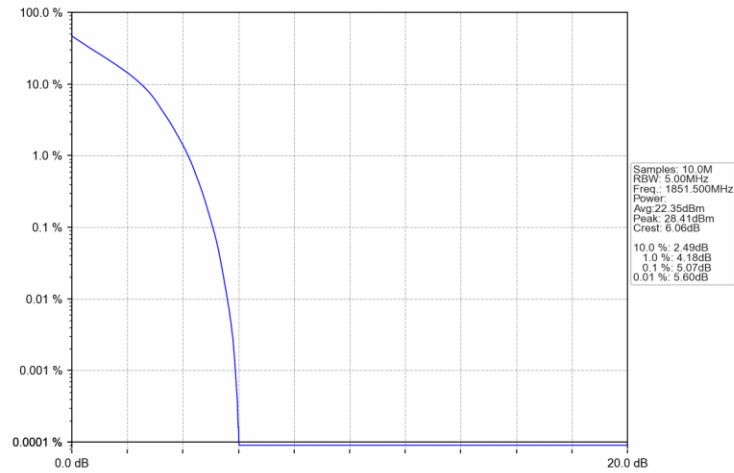
Band2 3MHz QPSK LCH 1851.5MHz RB 15 0 NTN
