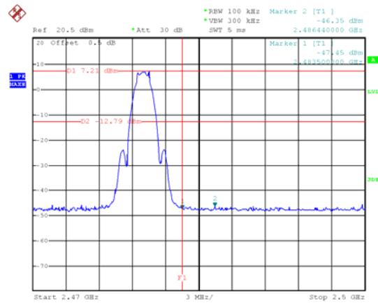
ZigBee: Band edge-right side
