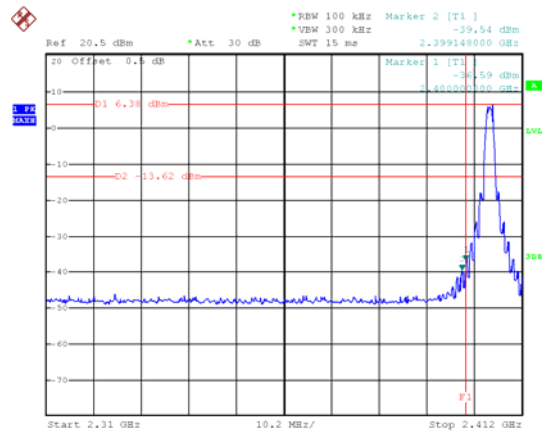
ZigBee: Band edge-left side
