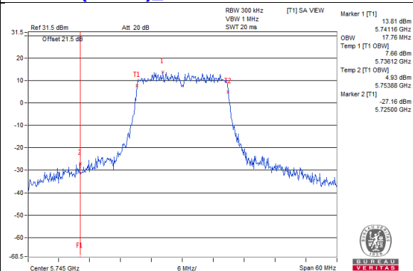
802.11ac(VHT20)_Chain2 / CH149
