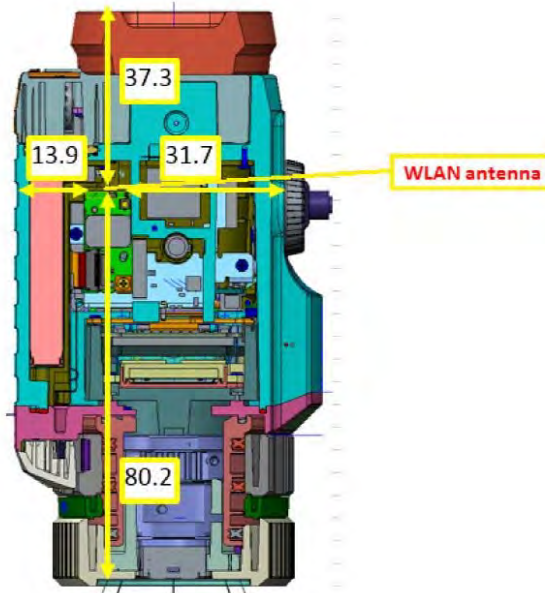
Fig.7 Antenna location
