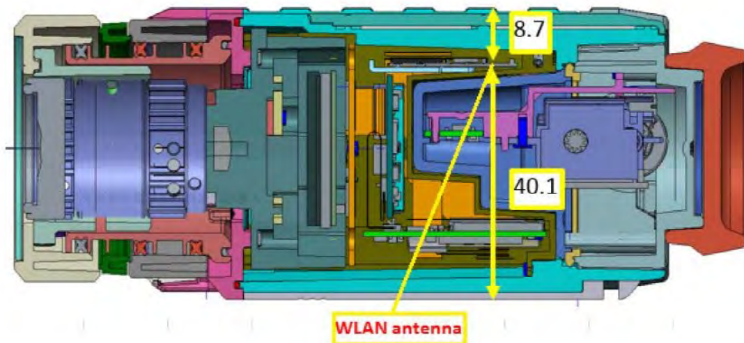
Fig.8 Antenna location
